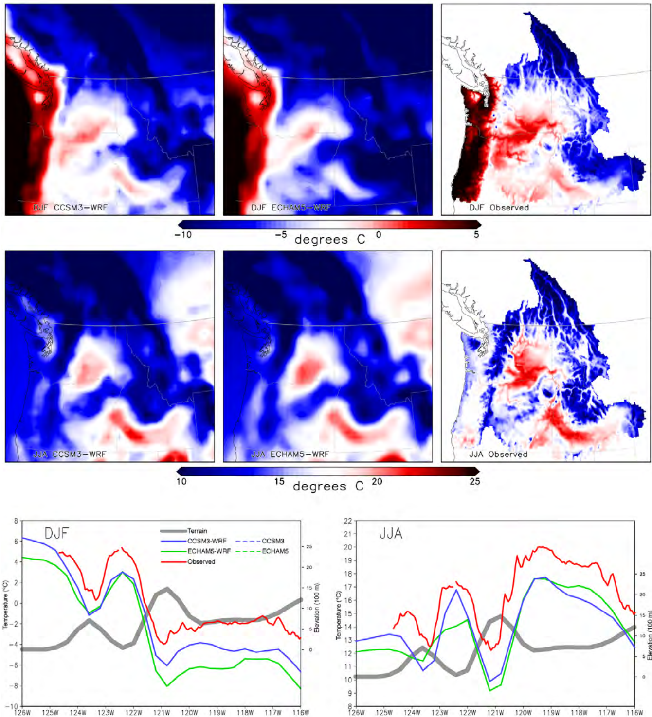
Figure 1. 1970-1999 seasonal mean temperature (°C) for DJF (top row) and JJA (middle row) from CCSM3-WRF (column 1), ECHAM5-WRF (column 2) and gridded observations (column 3). Bottom row: observed temperature and simulated temperature from both regional models and global forcing models along a West-East transect of the State of Washington at 47.8°N latitude. Terrain height is indicated by the thick gray line.
