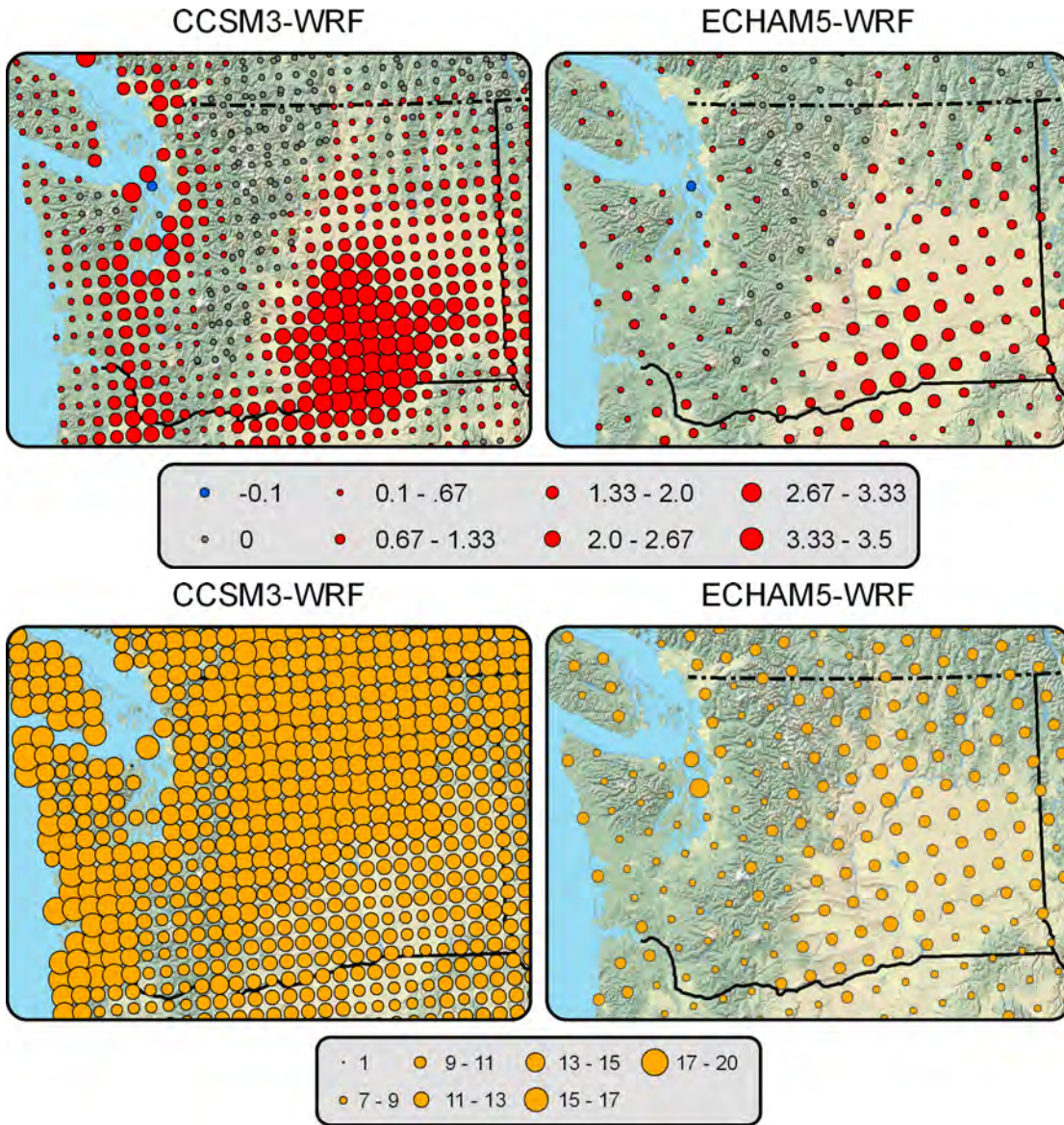
Figure 10. Top: change in the number of heat wave events from CCSM3-WRF (left) and ECHAM5-WRF (right). Bottom: change in the frequency of warm nights ( T_{min} > 90 th percentile).
