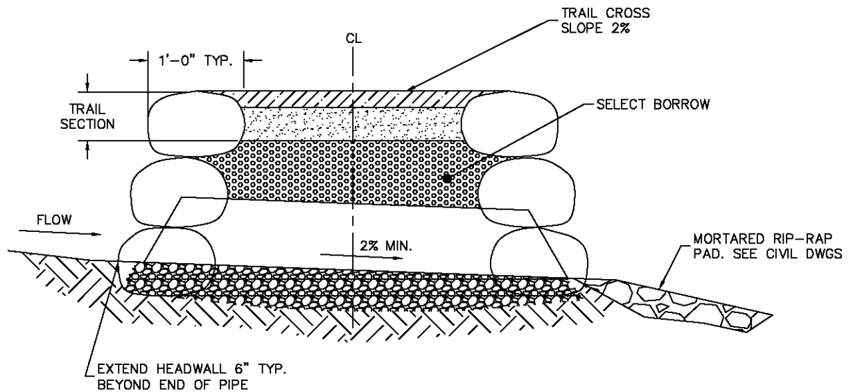
TRAIL SECTION VIEW
