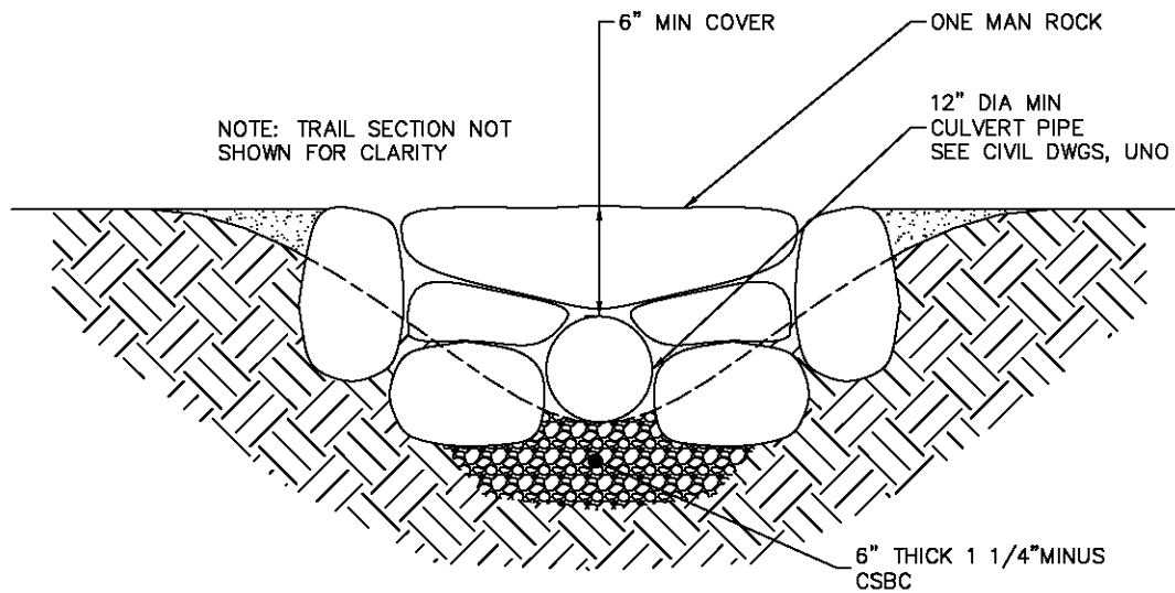
CULVERT SECTION VIEW
