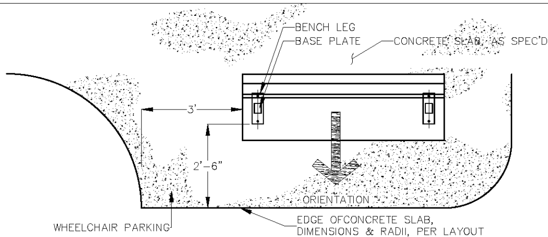
PLAN II W/ CONCRETE SLAB
