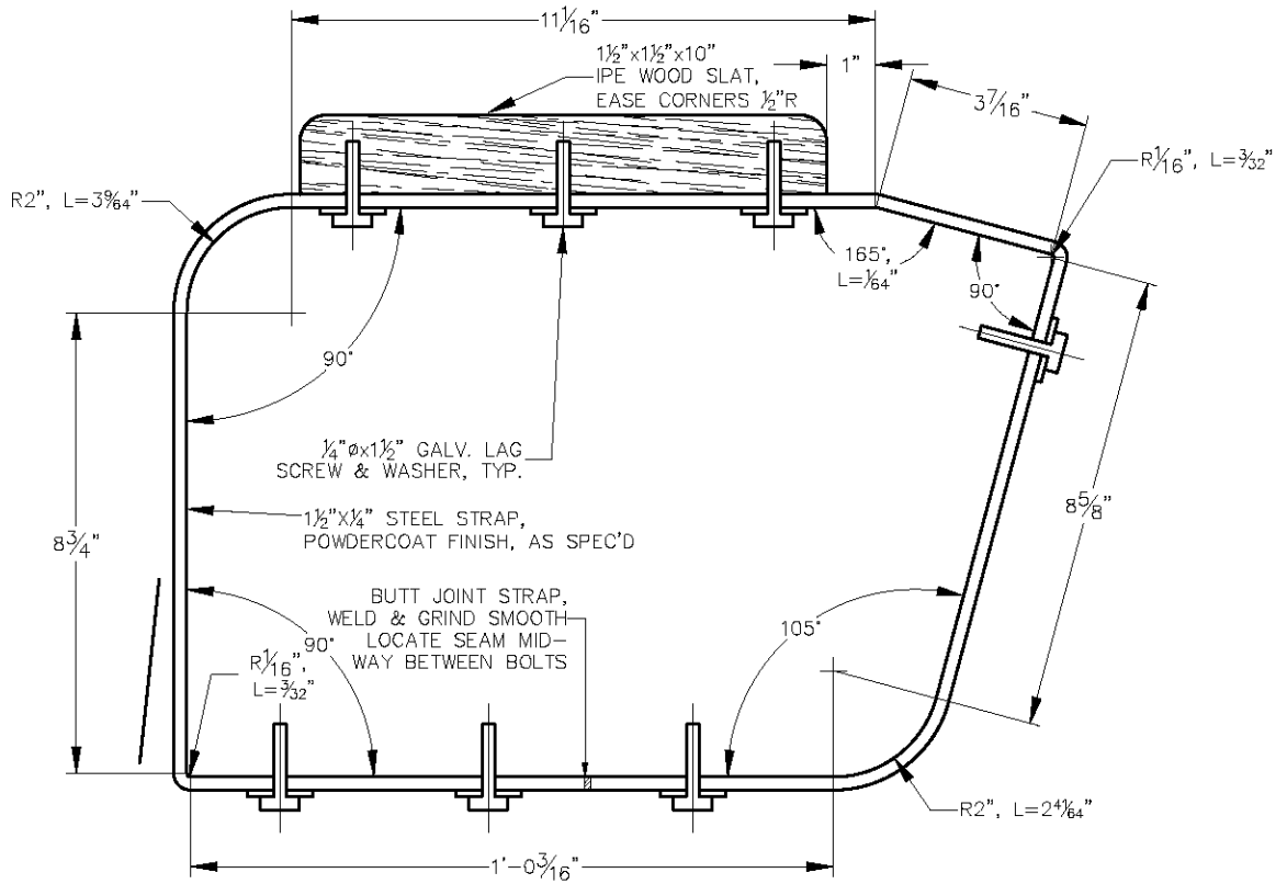
DETAIL-OPTIONAL ARMREST
