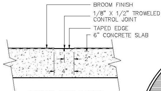
CONTROL JOINT & TAPED EDGE DETAIL SCALE: 1"=1'-0"
