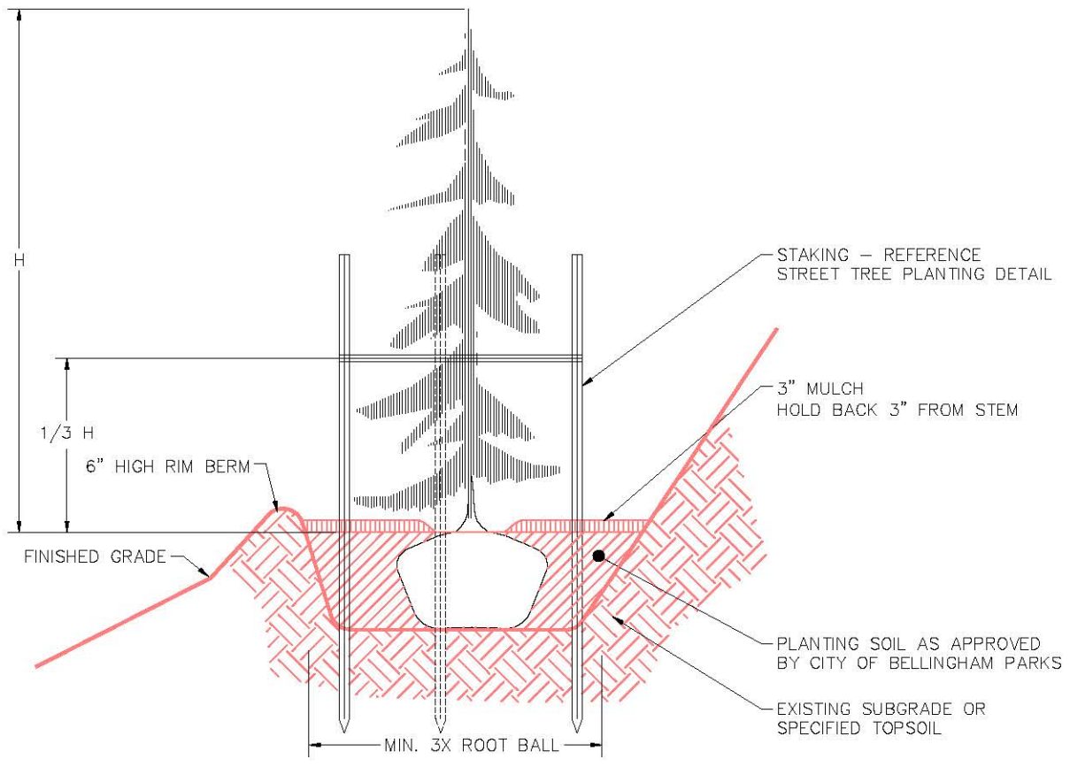
TREE PLANTING ON SLOPE
