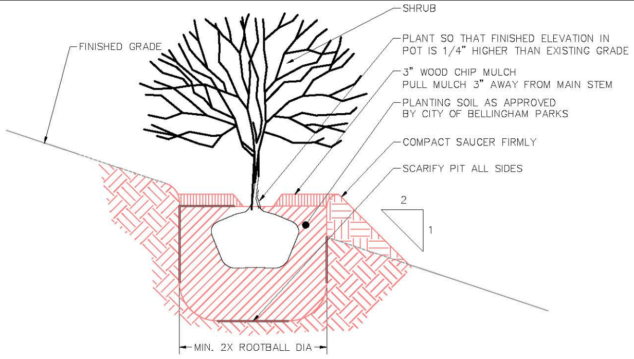
SHRUB PLANTING ON SLOPE
