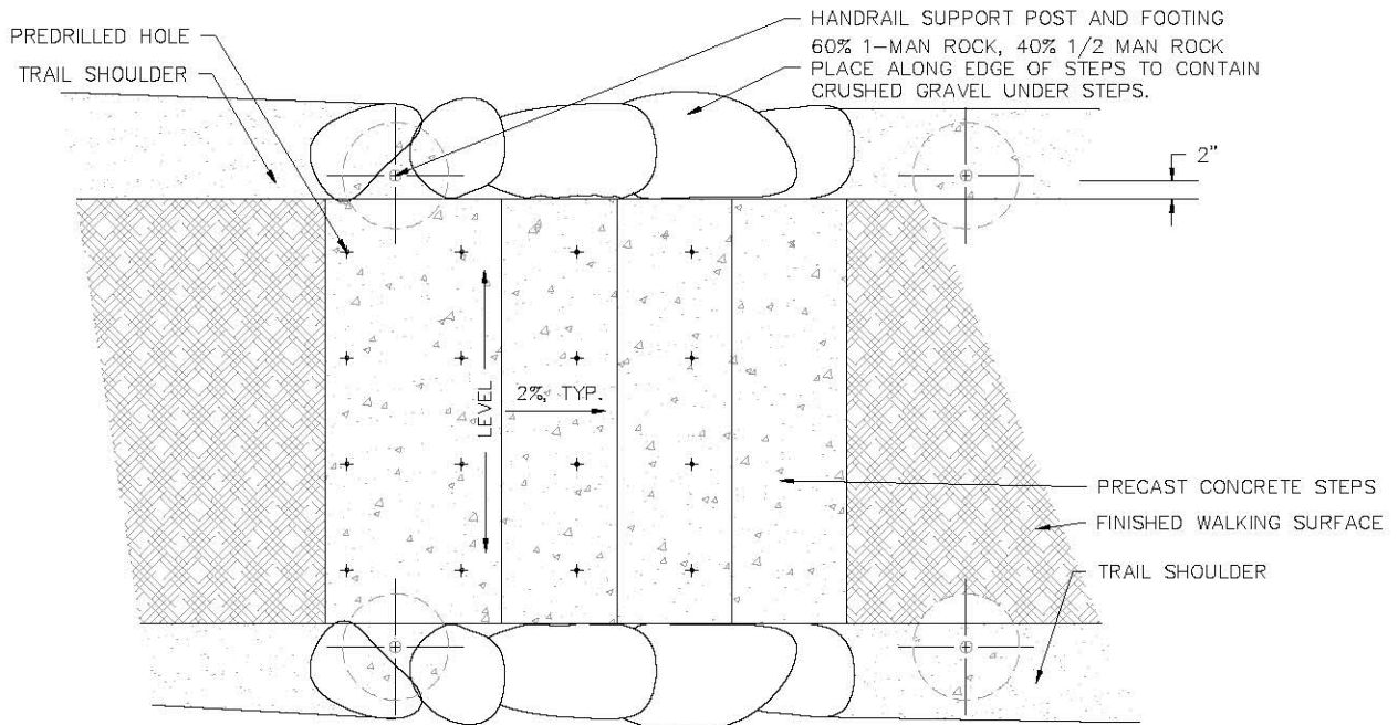
PLAN SCALE 1/2" = 1'-0"
