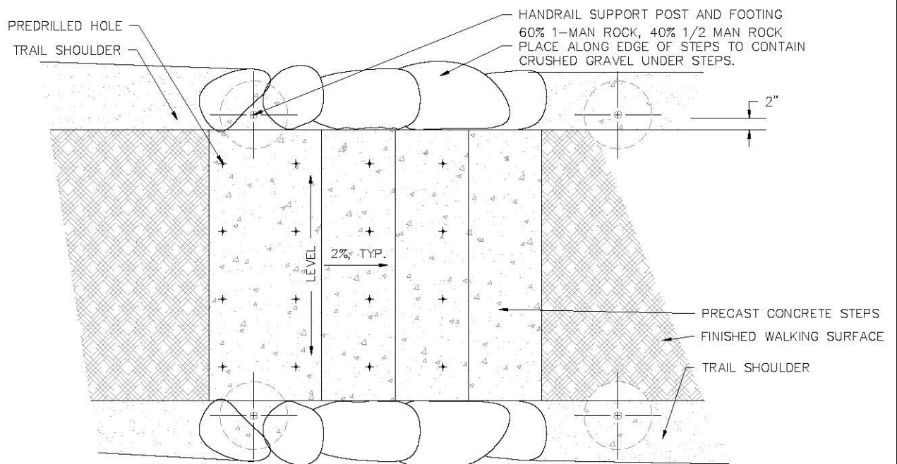
PLAN SCALE 1/2" = 1'-0"
