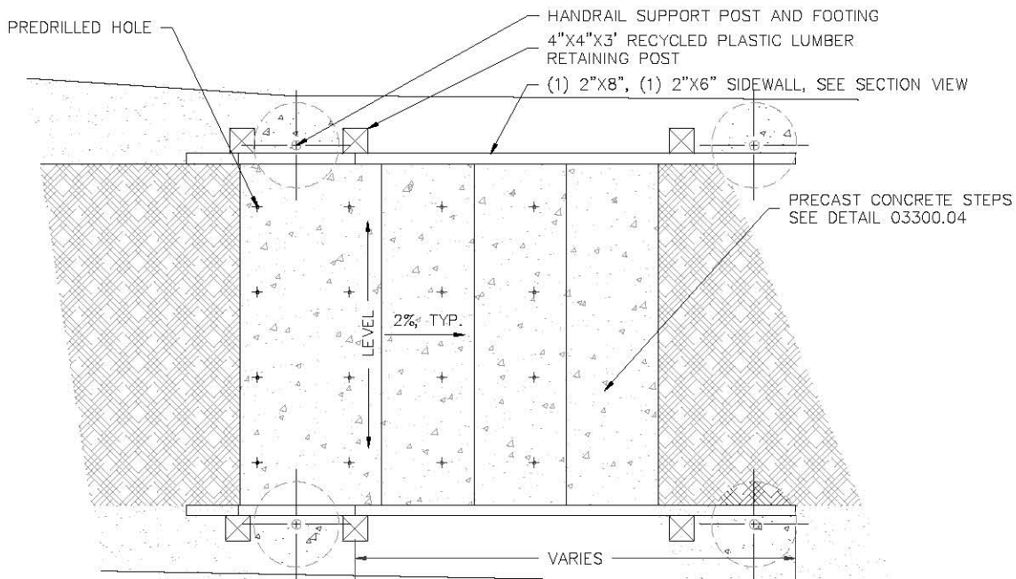
PLAN SCALE 1/2" = 1'-0"
