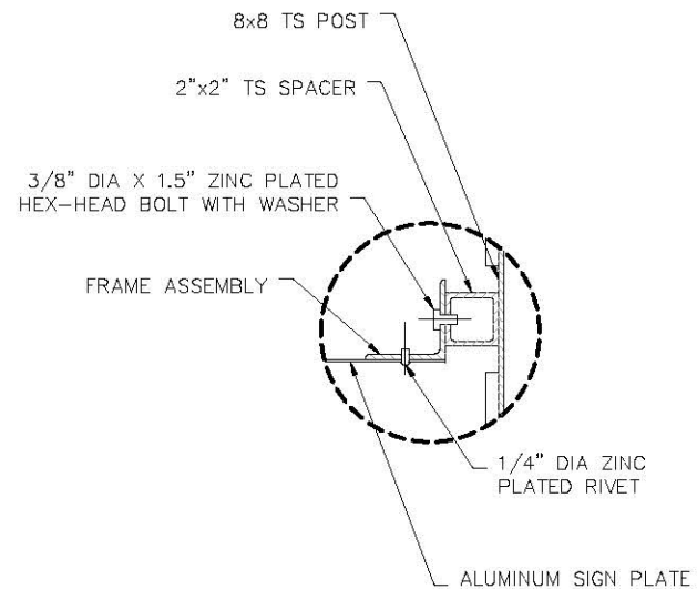
DETAIL A (SCALE 1-1/2" = 1'-0")
