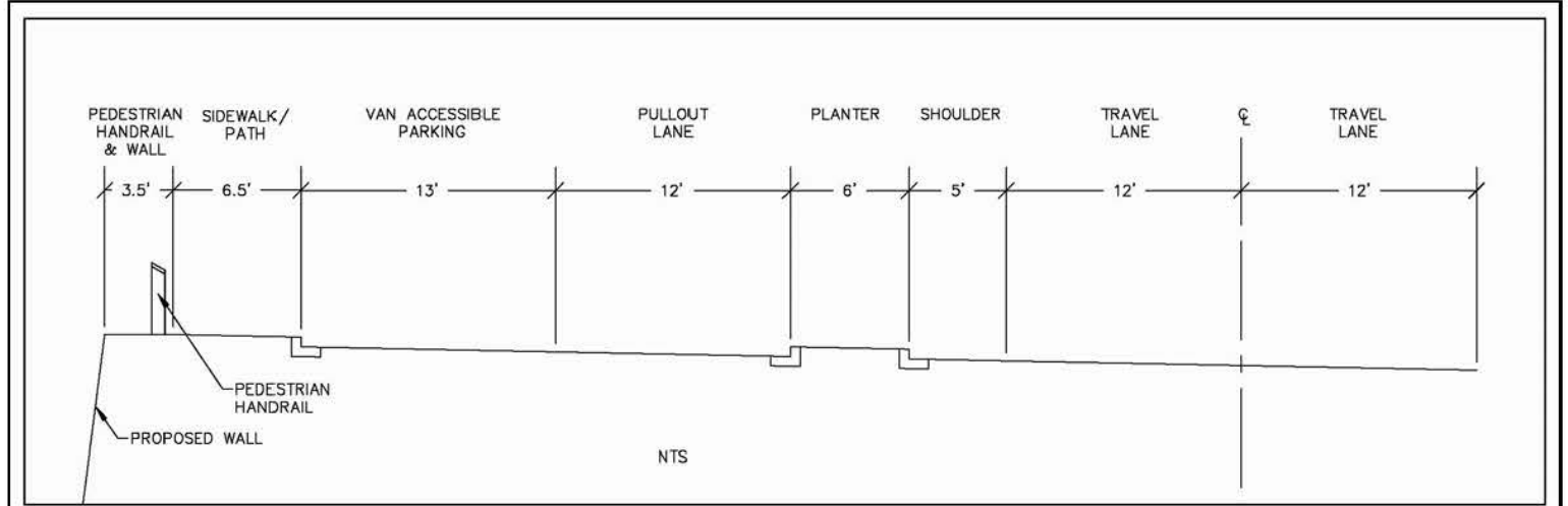
INSPIRATION POINT OVERLOOK SECTION
