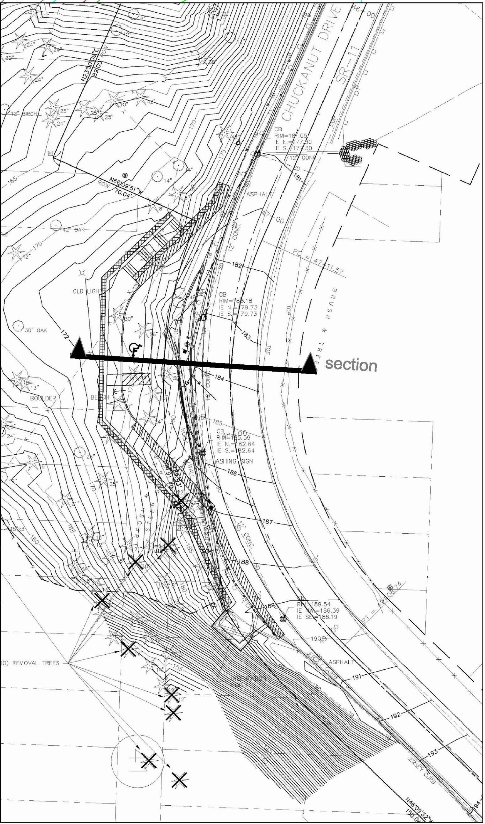
INSPIRATION POINT OVERLOOK PLAN
