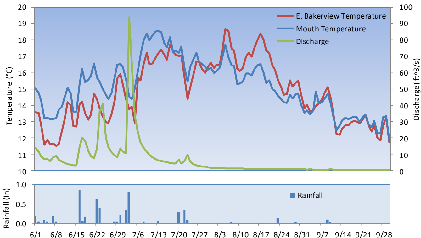
Figure 3.0-1. Effects of rain on flow and temperature levels in Padden Creek during the summer of 2012.
