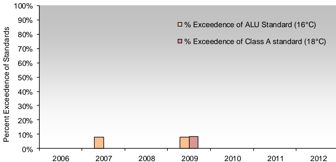
Figure 6.0-7. Percent of samples with temperatures in excess of the Core Summer Salmonid Habitat Aquatic Life Use (ALU) standard (16°C) for the Chuckanut Creek sampling site 2006 to 2012. The exceedence of the Class A (18°C) standard in 2009 is the only since 1998.
