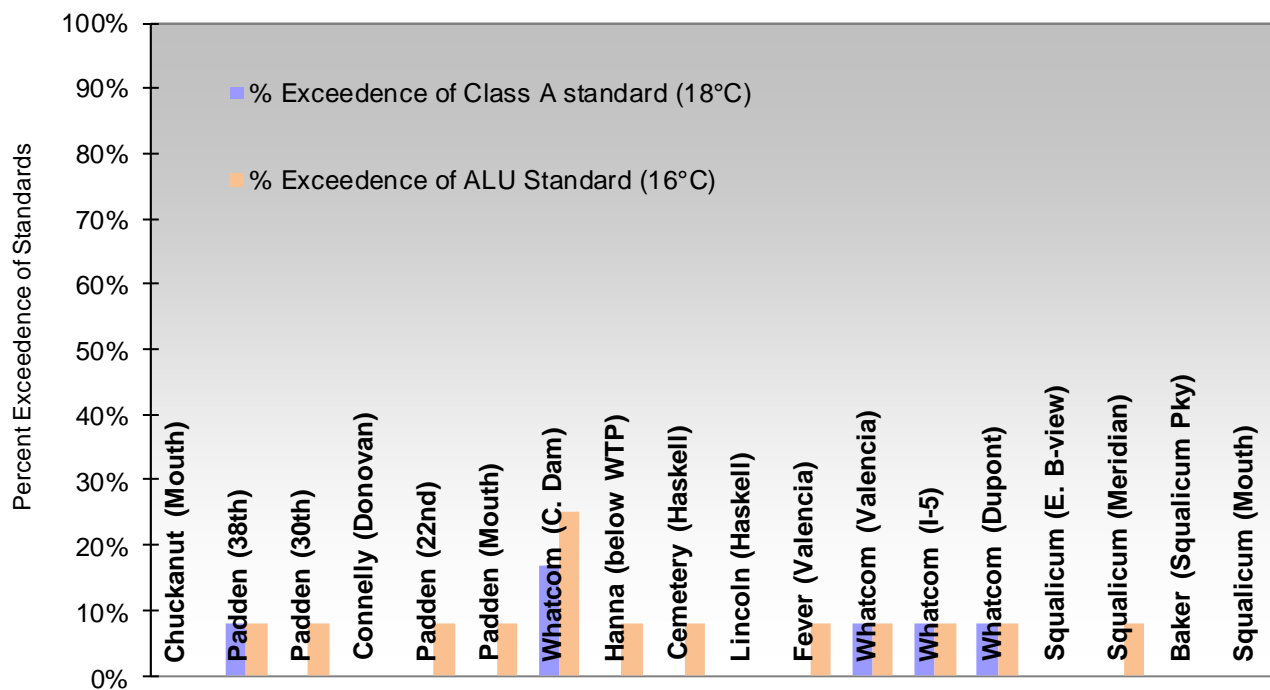
Figure 5.3.3-2. Percent temperature exceedences of Class A (18°C) and Aquatic Life Use (ALU, 16°C) standards for all stream segments sampled in 2012.
