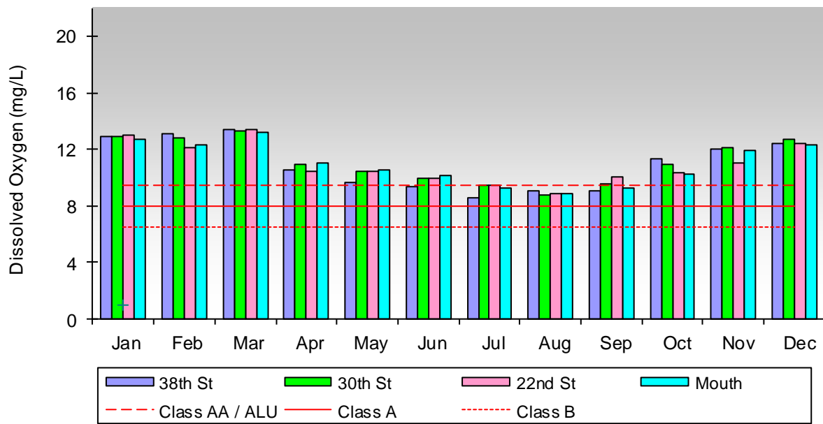
Figure 7.0-9. Dissolved oxygen for Padden Creek sampling sites by month in 2012. Red lines indicate the lowest dissolved oxygen levels allowed by the different surface water classes (Class AA, A, and B). Core Summer Salmonid Habitat Aquatic Life Use (ALU) is equivalent to Class AA.
