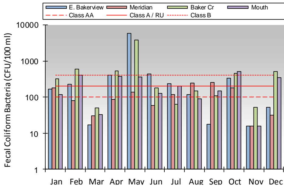
Figure 9.0-3. Monthly 2012 fecal coliform levels for sampling sites on Squalicum and Baker Creeks. Red lines indicate the numeric criteria for the calculated geomean for the different surface water classes (AA, A, and B). The Primary Contact Recreational Use (RU) designation is equivalent to Class A. Note this graph uses a logarithmic scale.
