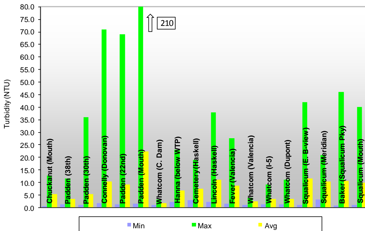
Figure 5.3.5-1. Minimum, maximum, and average turbidity values for all stream segments sampled in 2012.
