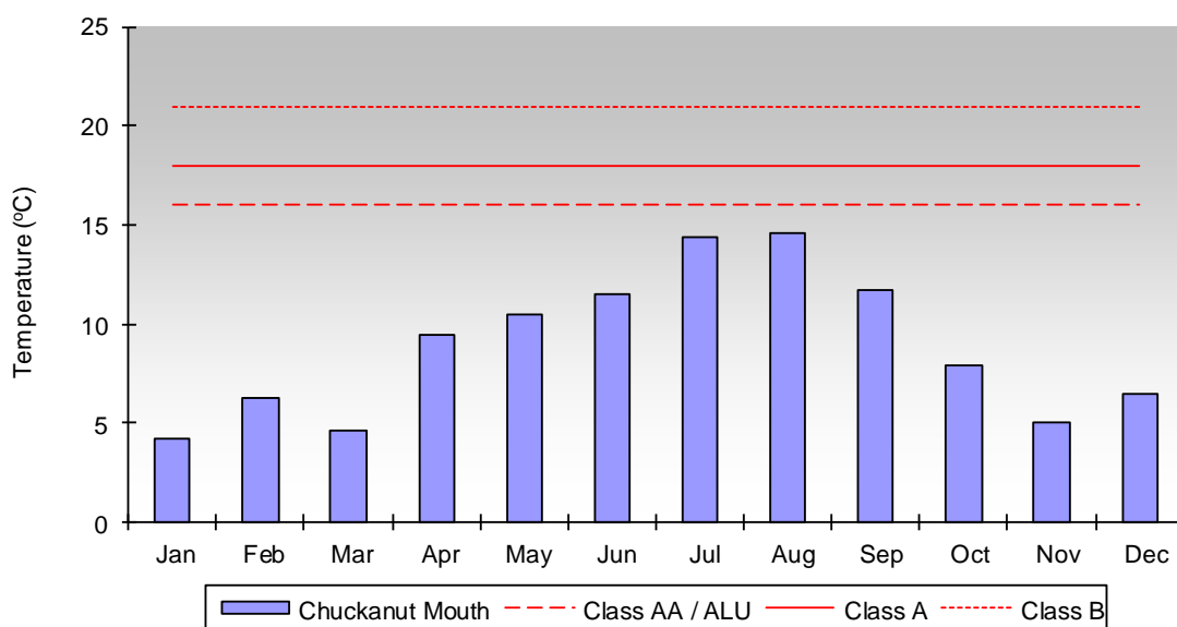
Figure 6.0-6. Monthly temperature measurements for the Chuckanut Creek sampling site in 2012. Red lines indicate the highest temperatures allowed by the different surface water standards (AA, A, and B). The Core Summer Salmonid Habitat ALU is equivalent to Class AA.
