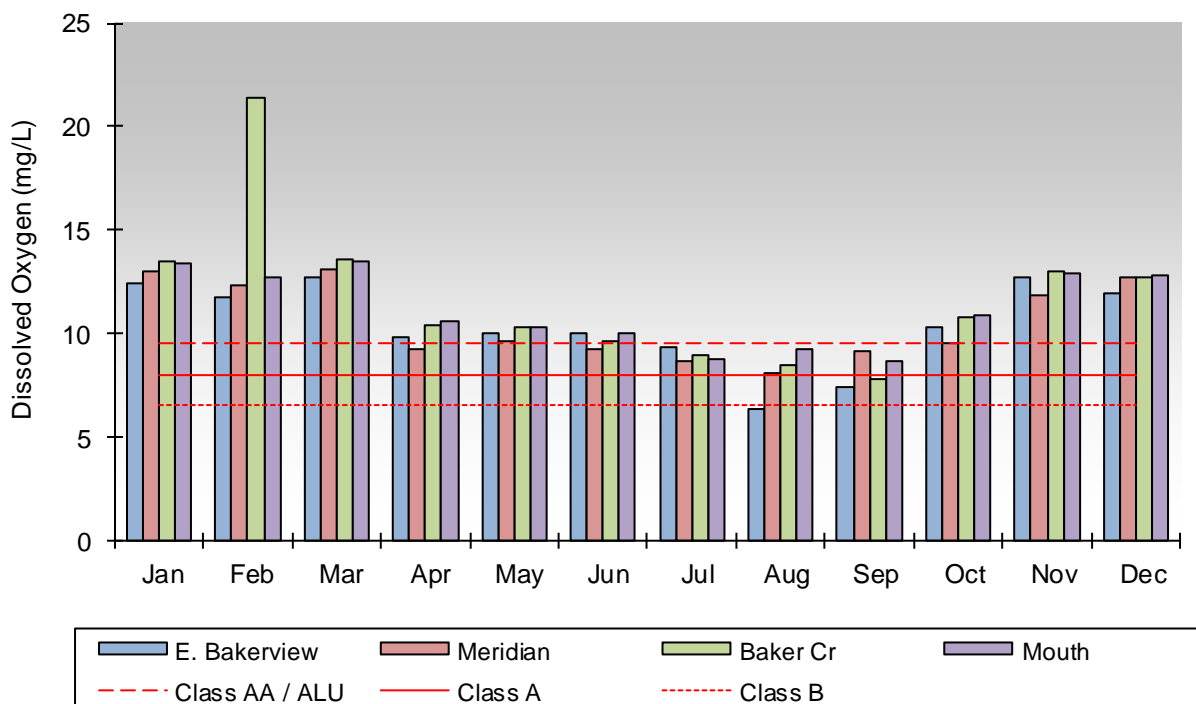
Figure 9.0-6. Monthly 2012 dissolved oxygen levels for Squalicum and Baker Creek sampling sites. Red lines the lowest dissolved oxygen levels allowed by the different surface water classes (AA, A, and B). Core Summer Salmonid Habitat Aquatic Life Use (ALU) is equivalent to Class AA. Based on conventional sampling.
