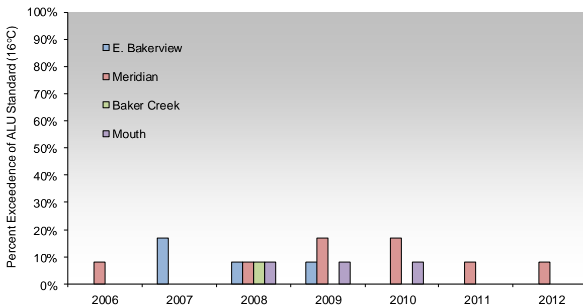
Figure 9.0-10. Percent of samples with temperatures in excess of the Core Summer Salmonid Habitat Aquatic Life Use (ALU) standard (16°C) for Squalicum and Baker Creek sampling sites 2006 to 2012. Results of conventional sampling indicate there have been no exceedences of the 18°C Class A standard since 1998. Gaps represent a 0% exceedence rate.
