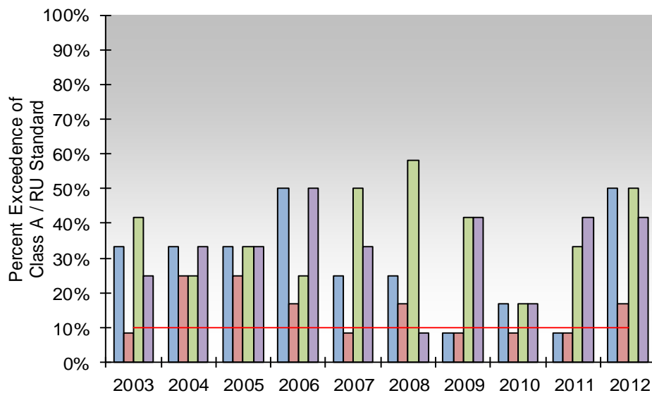
Figure 9.0-4 Percent exceedence of the Class A / RU standard for fecal coliform bacteria by year for Squalicum and Baker Creek sampling sites, 2003 to 2012. Gaps represent a 0% exceedence rate.
