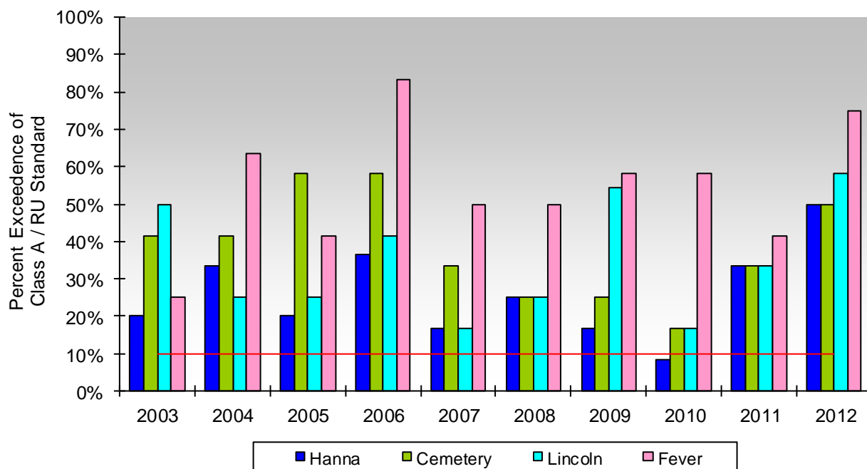
Figure 8.0-7a. Percent exceedence of the Class A / Recreational Use (RU) standard for fecal coliform bacteria by year for Whatcom Creek tributaries sampling sites, 2003 to 2012. Gaps represent a 0% exceedence rate.
