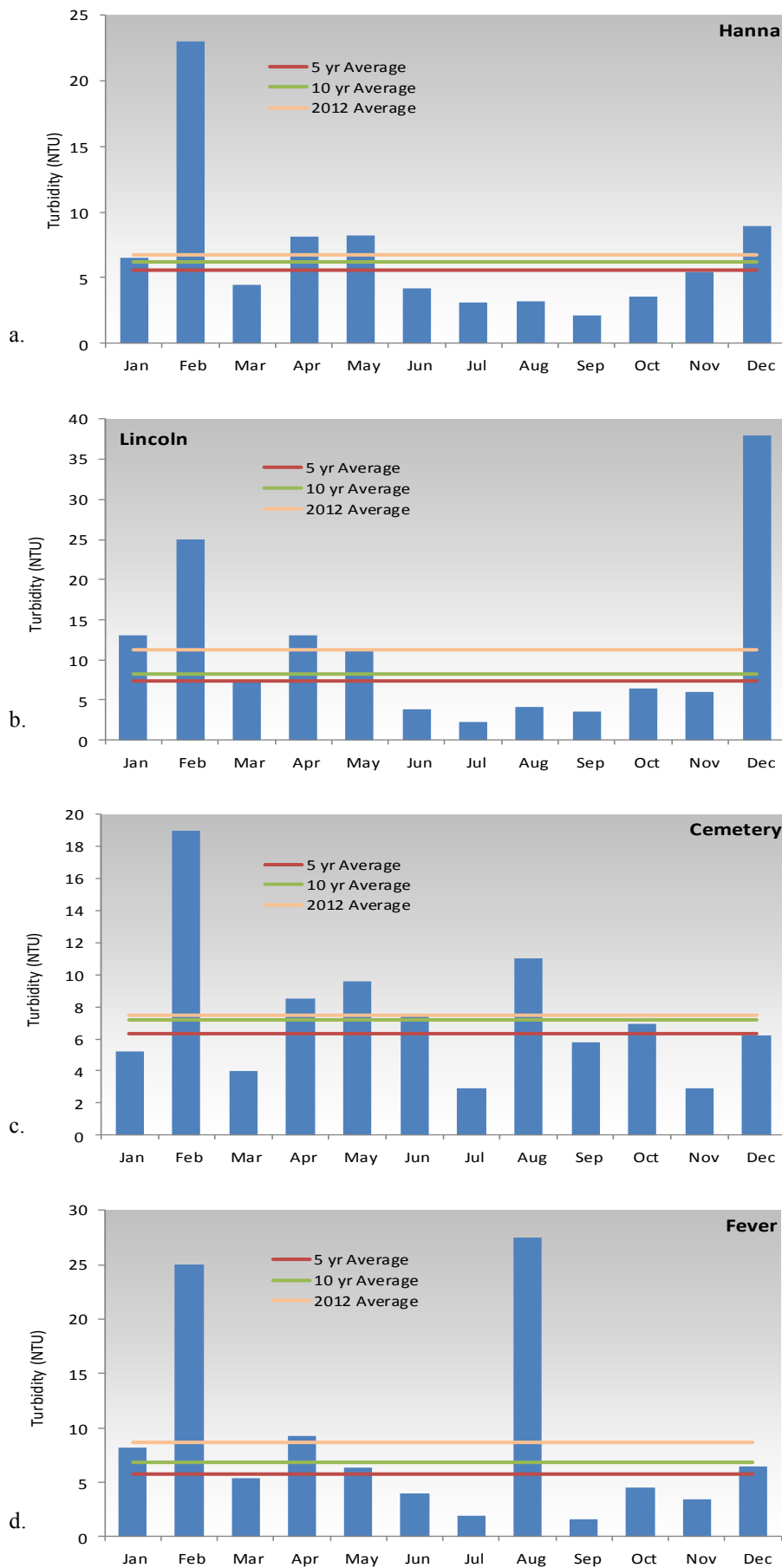
Figures 8.0-16a-d. Monthly turbidity values for Whatcom Creek tributaries in 2012. Presented with yearly, 5-year and 10-year averages.
