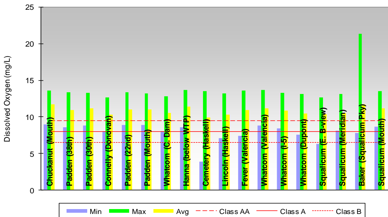
Figure 5.3.2-1. Minimum, maximum, and average dissolved oxygen levels for all stream segments sampled in 2012. Red lines indicate the lowest dissolved oxygen levels allowed for the different surface water classes (AA, A, and B). The Core Summer Salmonid Habitat Aquatic Life Use (ALU) designation is equivalent to Class AA.
