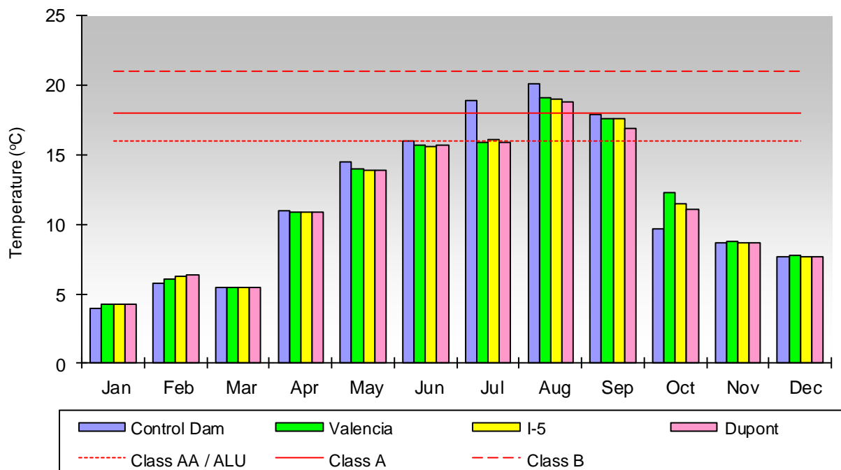
Figure 8.0-13. Monthly temperature measurements for Whatcom Creek sampling sites in 2012. Red lines indicate the highest temperatures allowed by the different surface water standards (Class AA, A, and B). Core Summer Salmonid Habitat Aquatic Life Use (ALU) is equivalent to Class AA.
