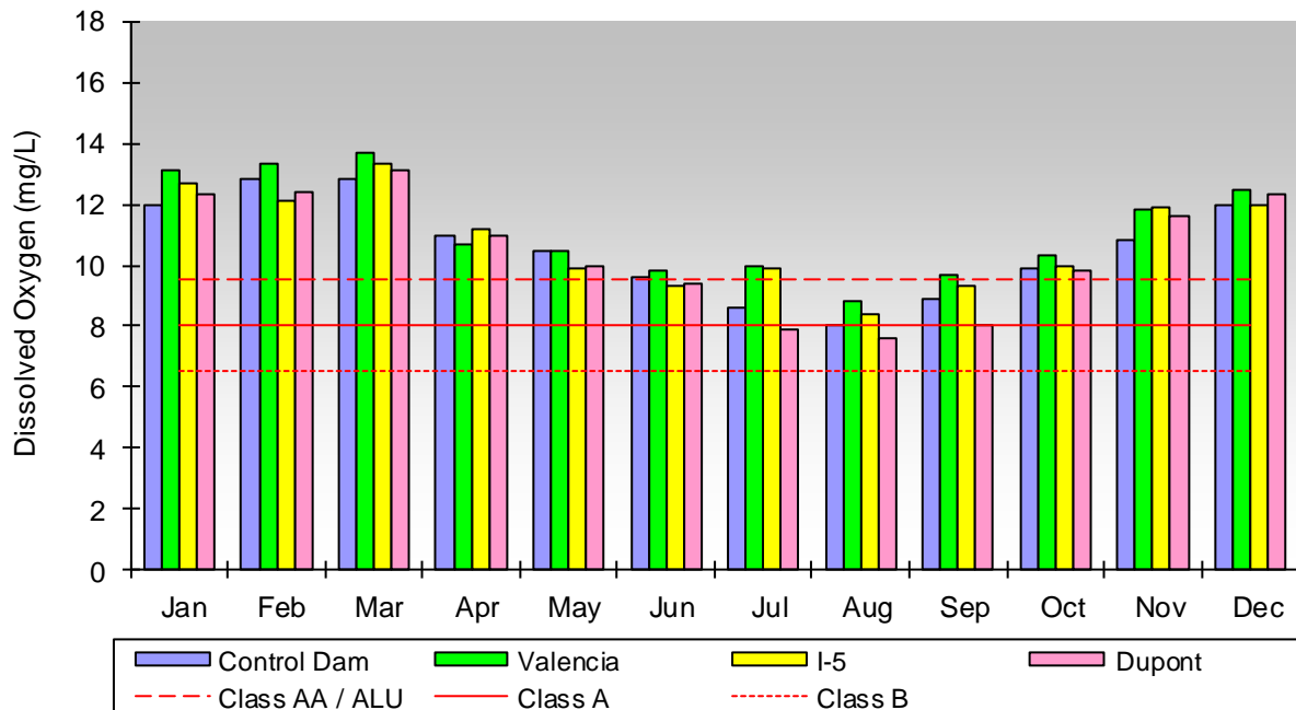
Figure 8.0-9. Monthly 2012 dissolved oxygen levels for Whatcom Creek sampling sites. Red lines indicate the lowest dissolved oxygen levels allowed by the different surface water classes (AA, A, and B). Core Summer Salmonid Habitat Aquatic Life Use (ALU) is equivalent to Class AA.
