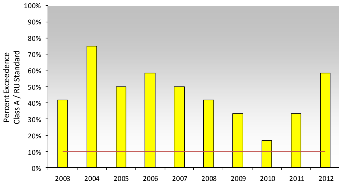
Figure 7.0-4a. Percent exceedence of the Class A / Recreational Use (RU) standard for fecal coliform bacteria by year for Connelly Creek, 2003 to 2012.
