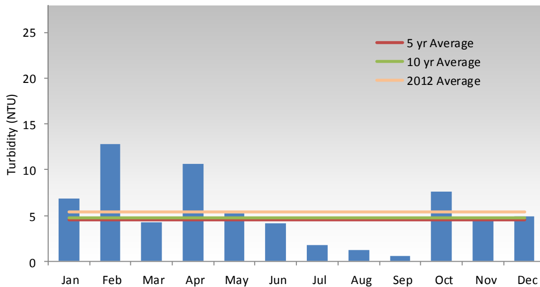
Figure 6.0-8. Monthly turbidity values and yearly averages for the Chuckanut Creek sampling site in 2012. Presented with yearly, 5-year and 10-year averages.
