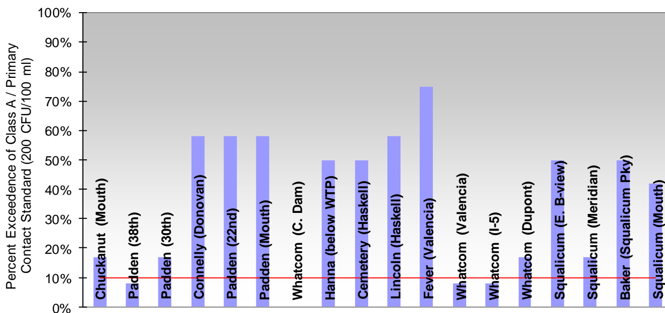
Figure 5.3.1-2. Fecal coliform percent exceedence of the Class A / Primary Recreational Contact standard for all stream segments sampled in 2012. Whatcom Creek at the Control Dam had no exceedences for 2012. Based on conventional sampling events.
