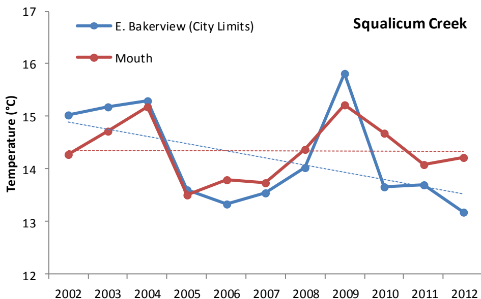
Figures 1.2-1 and 1.2-2. Mean critical period (June 1 - October 1) temperatures at the headwater/city limits and mouth sites on Padden and Squalicum Creeks, 2002 – 2012.
