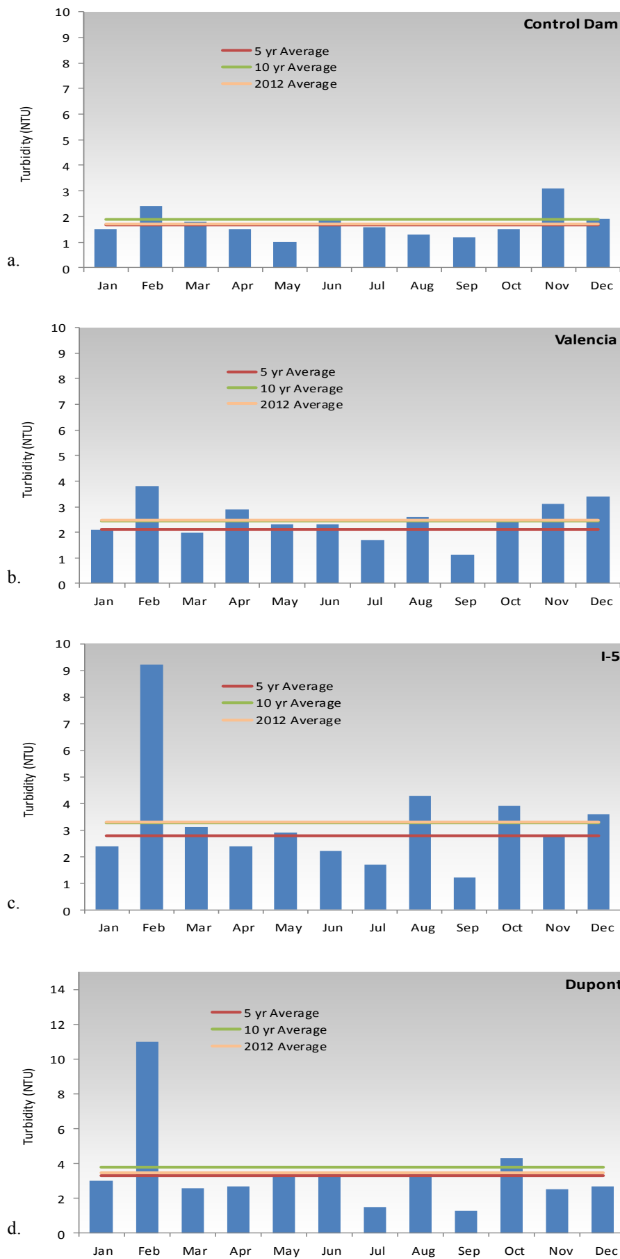
Figures 8.0-15a-d. Monthly turbidity values for Whatcom Creek Sampling sites in 2012. Presented with yearly, 5-year and 10-year averages.
