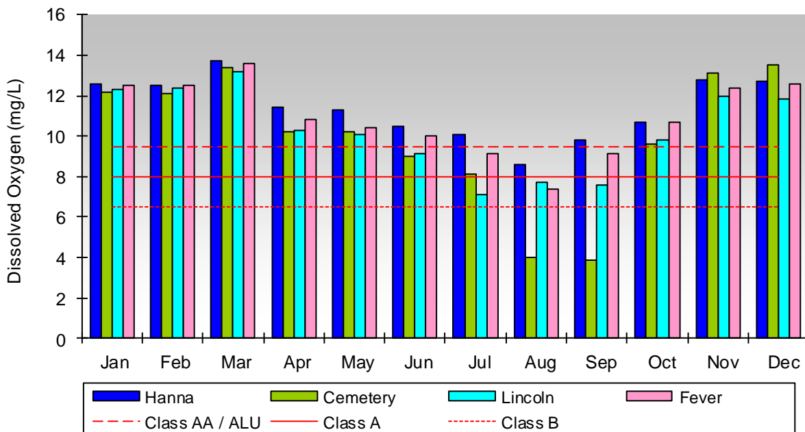
Figure 8.0-9a. Monthly 2012 dissolved oxygen levels for Whatcom Creek tributaries sampling sites. Red lines indicate the lowest dissolved oxygen levels allowed by the different surface water classes (AA, A, and B). Core Summer Salmonid Habitat Aquatic Life Use (ALU) is equivalent to Class AA.
