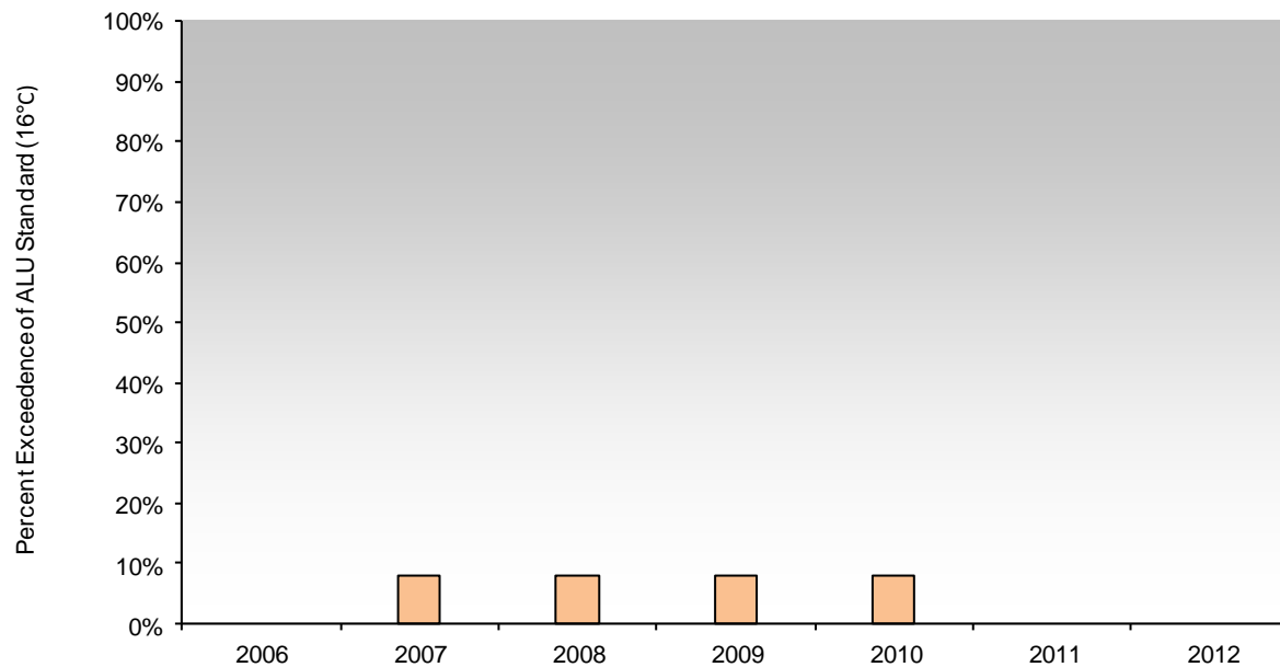
Figure 7.0-12a. Percent of samples with temperatures in excess of the Core Summer Salmonid Habitat Aquatic Life Use (ALU) standard (16°C) for the Connelly Creek sampling site 2006 to 2012. There have been no exceedences of the Class A (18°C) standard since 1998. Gaps in graph represent a 0% exceedence rate.
