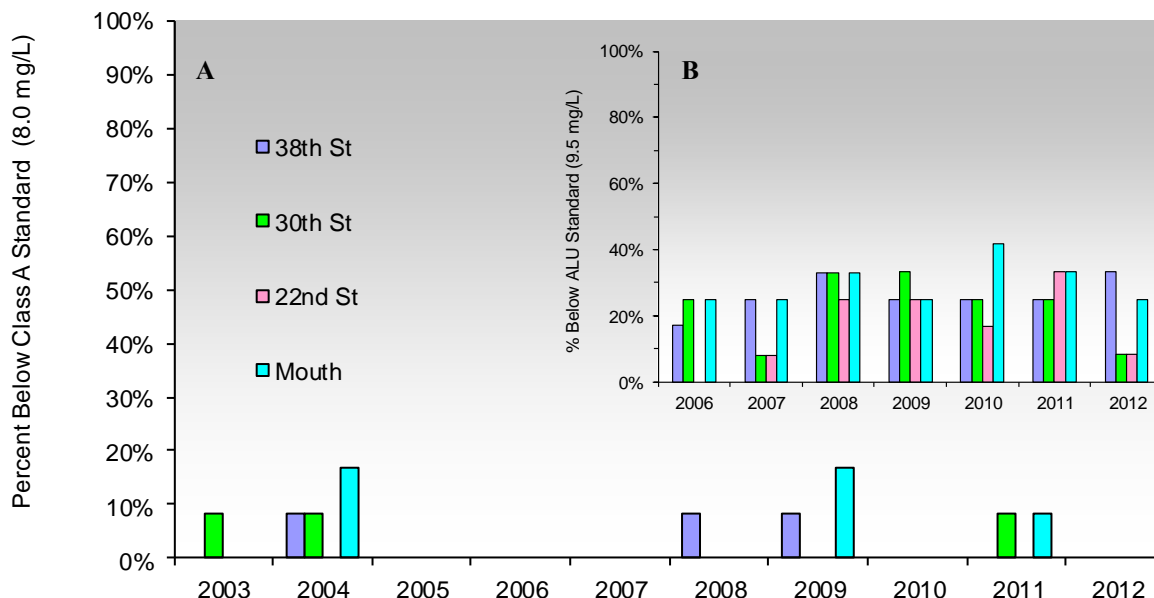
Figure 7.0-10. A. Percent of dissolved oxygen samples below the Class A standard (8.0 mg/L) for Padden Creek sampling sites 2003 to 2012. B. Percent of dissolved oxygen samples below the Core Summer Salmonid Habitat Aquatic Life Use (ALU) designation (9.5 mg/L) from 2006-2012. Sampling began on 22 nd St. in 2005. All other gaps in graph represent a 0% rate of samples below standards.
