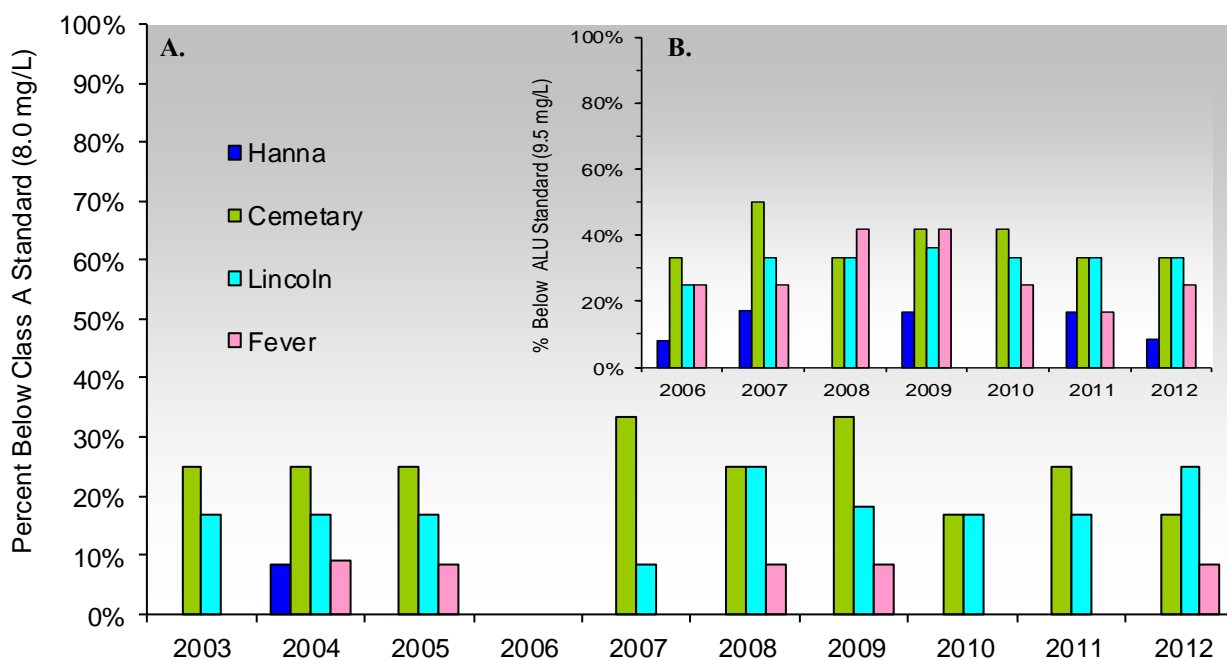
Figure 8.0-10a. A. Percent of dissolved oxygen samples below 8.0 mg/L for Whatcom Creek tributaries sampling sites 2003 to 2012. B. Percent of dissolved oxygen samples below the Core Summer Salmonid Habitat Aquatic Life Use (ALU) designation (9.5 mg/L) from 2006-2012. Gaps represent a 0% rate of samples below standards.
