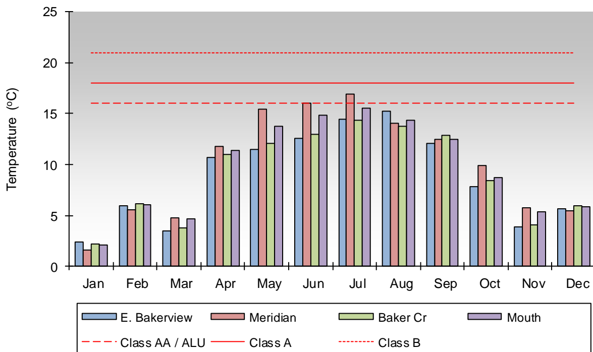
Figure 9.0-9. Monthly temperature measurements for Squalicum and Baker Creek sampling sites in 2012. Red lines indicate the highest temperatures allowed by the different surface water standards (AA, A, and B). Core Summer Salmonid Habitat Aquatic Life Use (ALU) is equivalent to Class AA. Based on conventional sampling.
