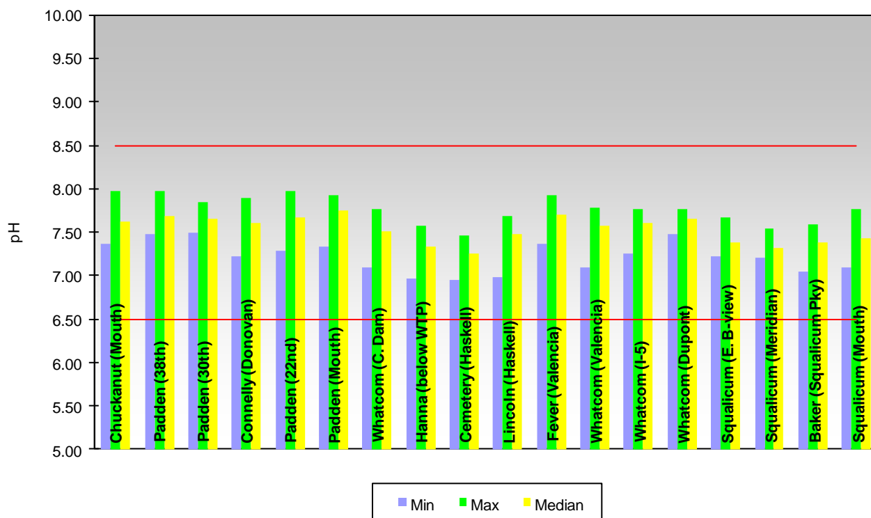
Figure 5.3.4-1. The pH minimum, maximum, and median values for all stream segments sampled in 2012. Red lines indicate the minimum and maximum values allowed by the Class AA/A/B and Aquatic Life Use (ALU) criteria for pH.
