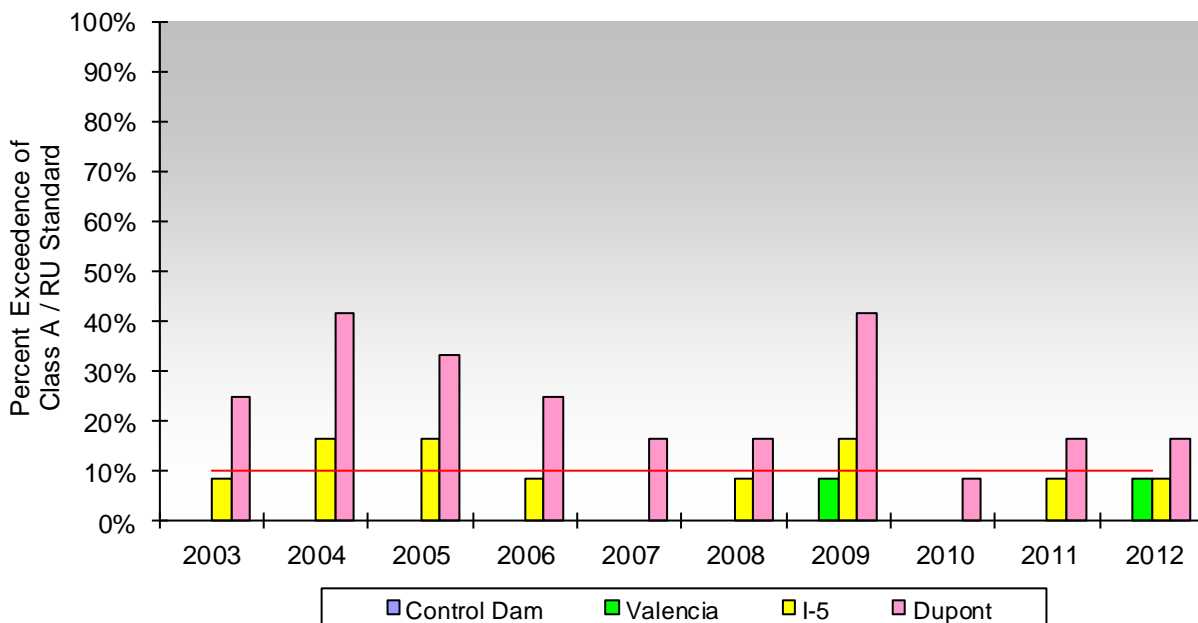
Figure 8.0-7. Percent exceedence of the Class A / Recreational Use (RU) standard for fecal coliform bacteria by year for Whatcom Creek sampling sites, 2003 to 2012. Sampling at Valencia began in 2007. Gaps represent a 0% exceedence rate.
