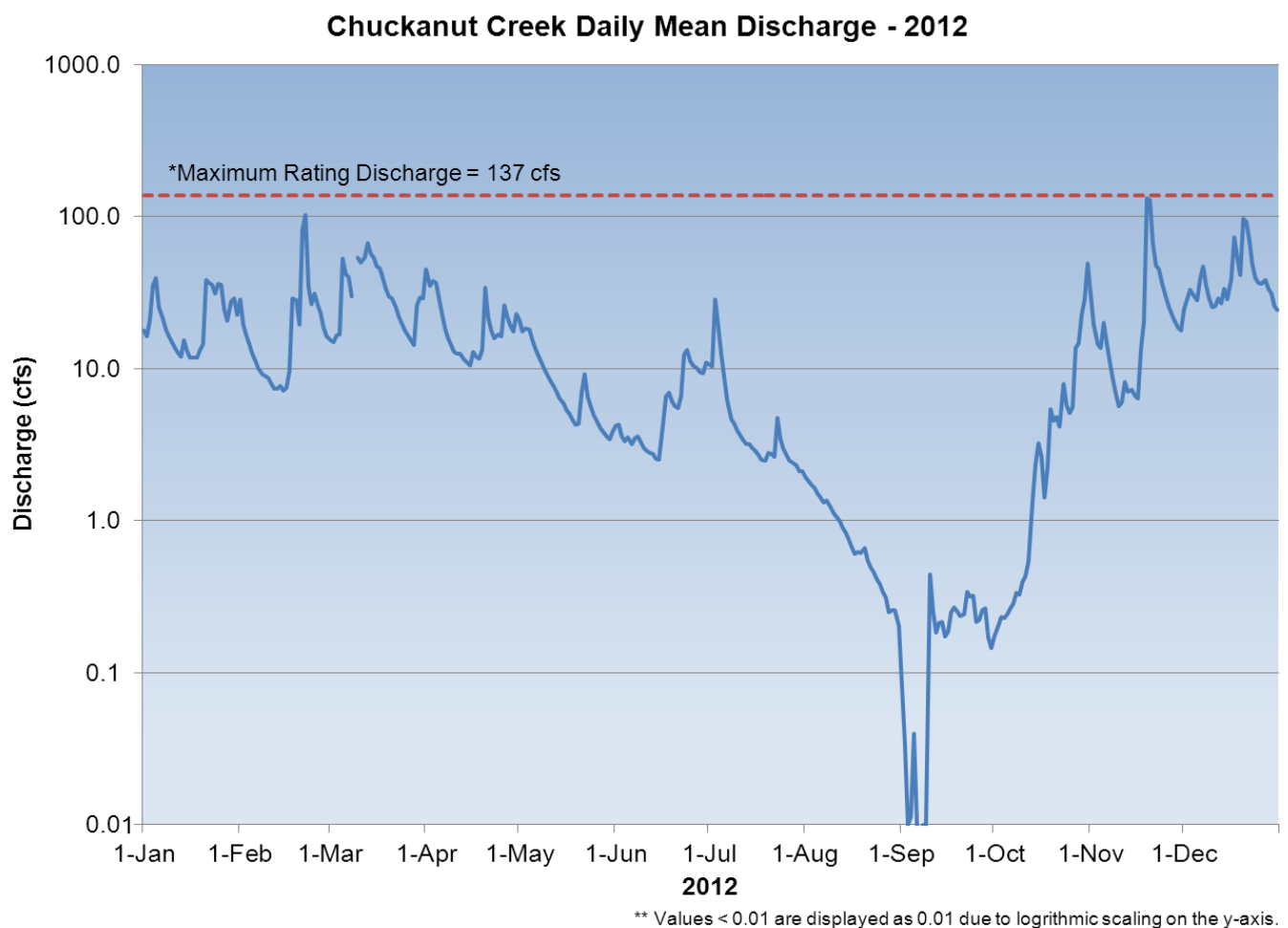
Figure 6.0-9. Daily mean discharge on Chuckanut Creek during 2012. Discharge values above the maximum rating discharge of 137 cfs are of poor quality and should be interpreted cautiously. This hydrograph uses a logarithmic scale.
