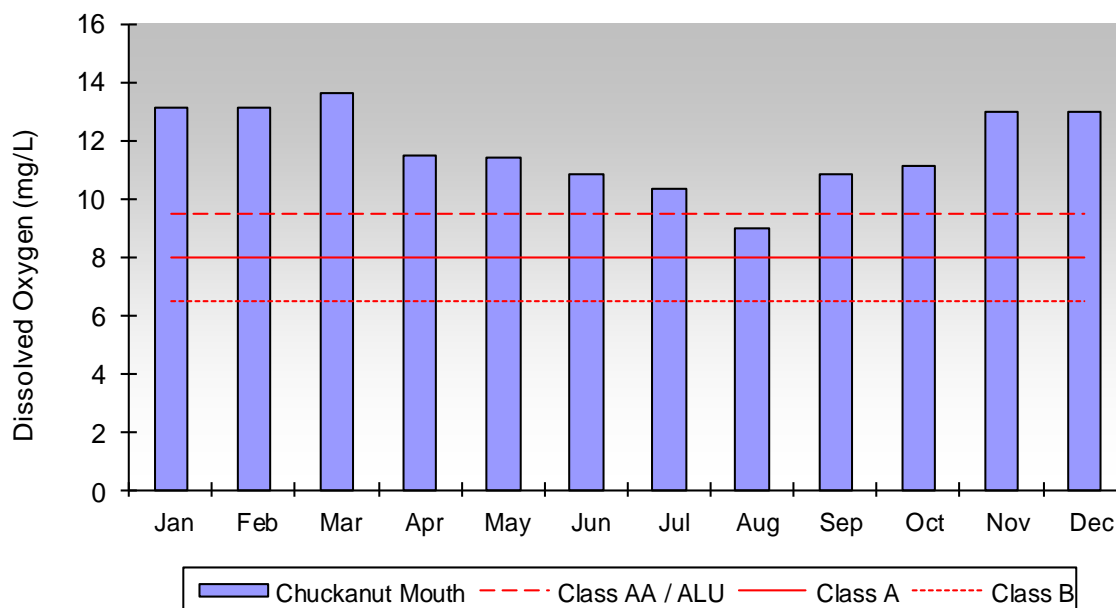
Figure 6.0-4. Monthly 2012 dissolved oxygen levels for Chuckanut Creek. Red lines indicate the lowest dissolved oxygen levels allowed by the different surface water standards (AA, A, and B). Core Summer Salmonid Habitat Aquatic Life Use (ALU) is equivalent to Class AA.
