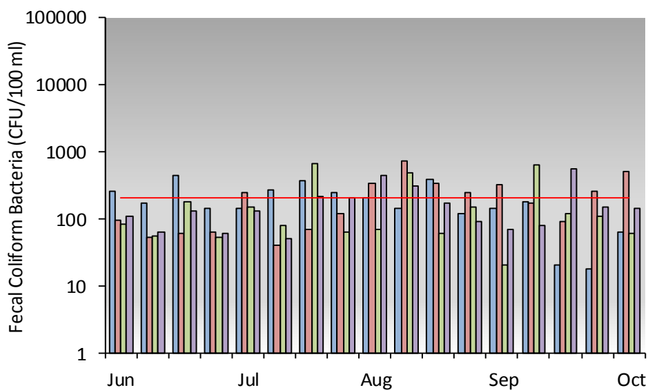
Figure 9.0-5. Fecal coliform levels during enhanced sampling June - October 2012.
