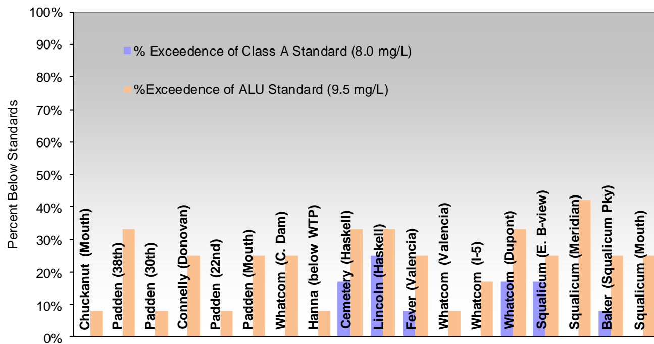
Figure 5.3.2-2. Percent of dissolved oxygen samples below the Class A (8.0 mg/L) and Aquatic Life Use (ALU, 9.5 mg/L) standards for all stream segments sampled in 2012.
