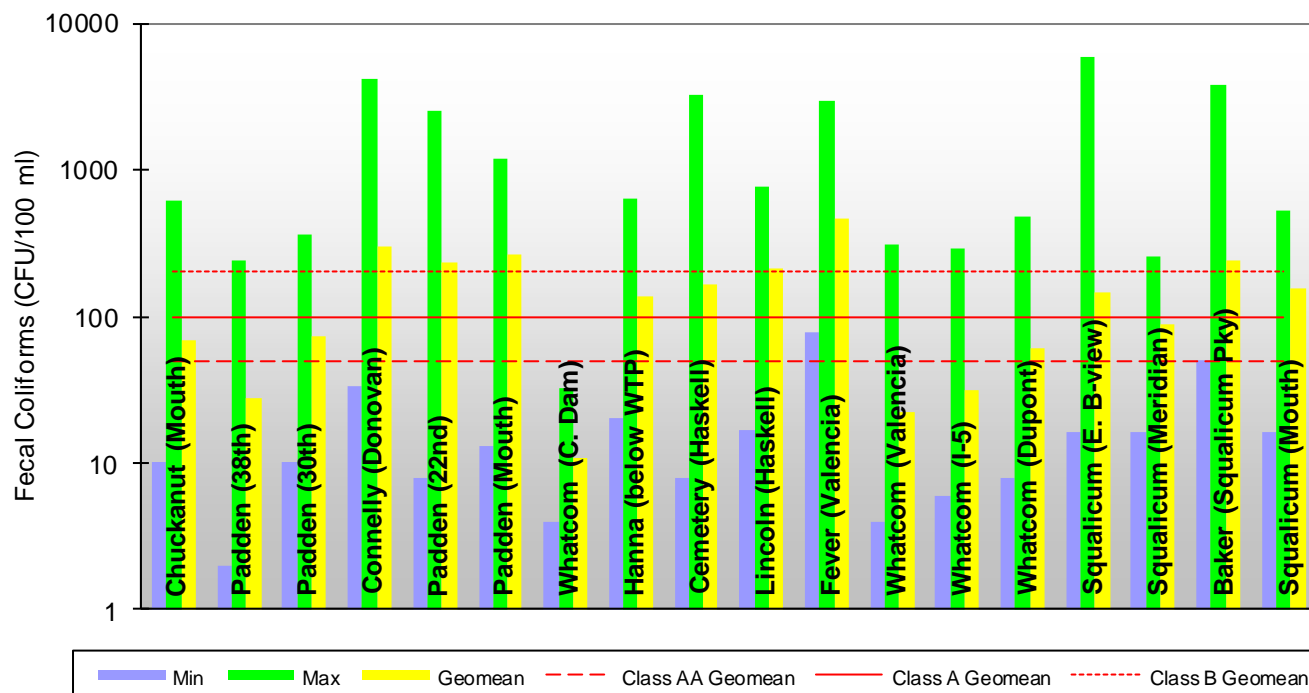
Figure 5.3.1-1. Fecal coliform bacteria minimum, maximum, and geomean values for all stream segments sampled in 2012. Red lines indicate the maximum geomean value allowed by the Class AA, A (Primary Recreational Contact), and B criteria for fecal coliform bacteria. Note this graph uses a logarithmic scale.
