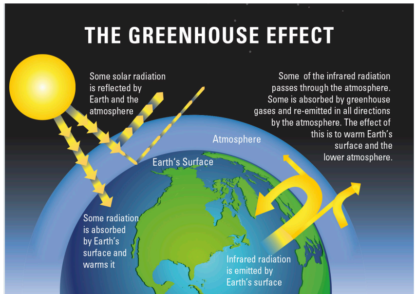
Figure 3. The greenhouse effect (USGCRP 2014)
