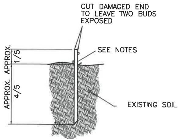
TYPICAL LIVE STAKE INSTALLATION
