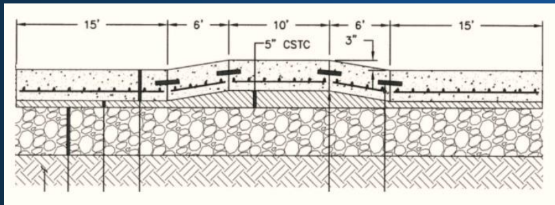
Cross-section of a Speed Table
