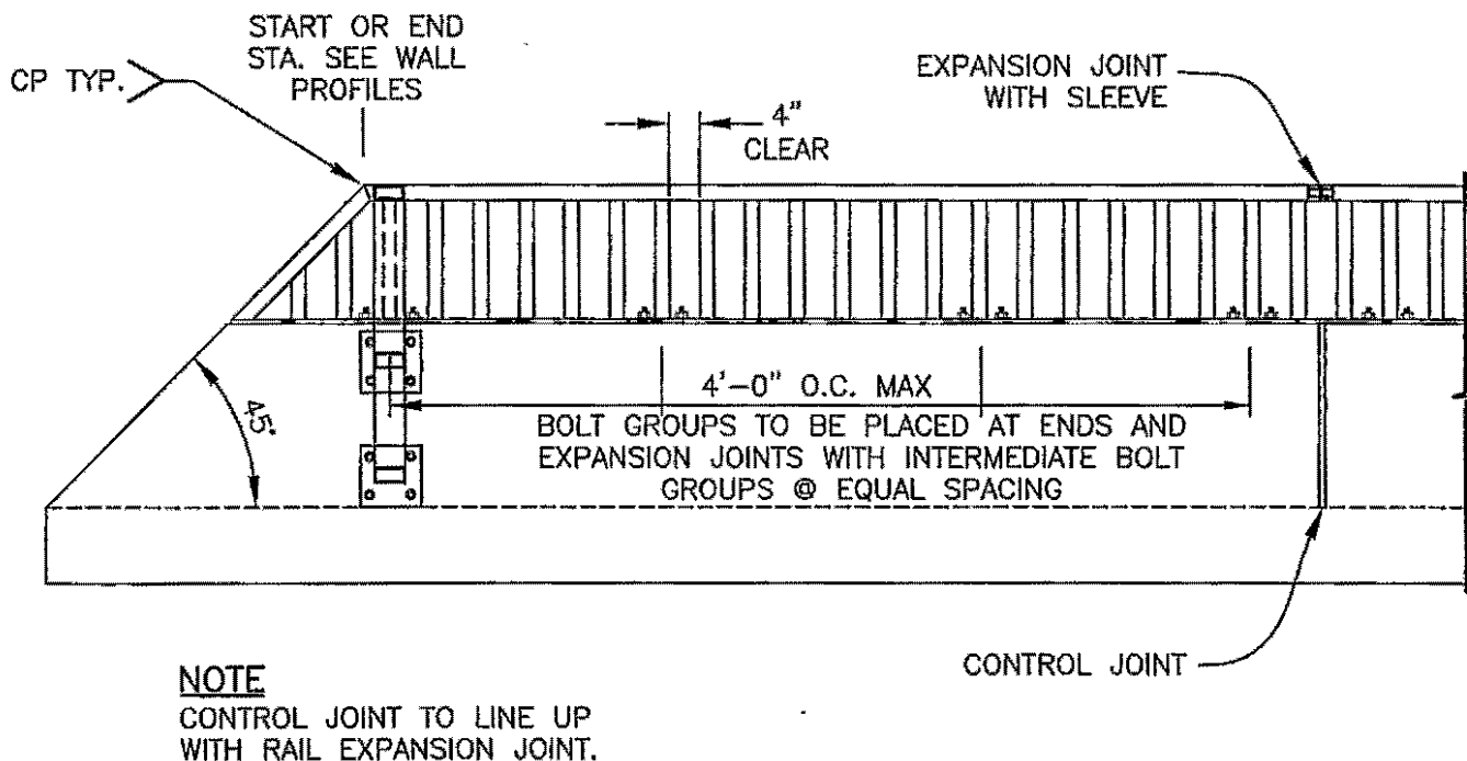
BARRIER RAIL ELEVATION N.T.S.
