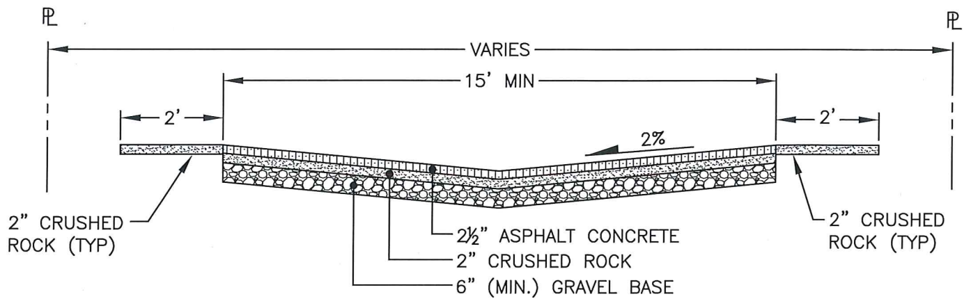
ALTERNATE A ASPHALT CONCRETE ALLEY PAVEMENT
