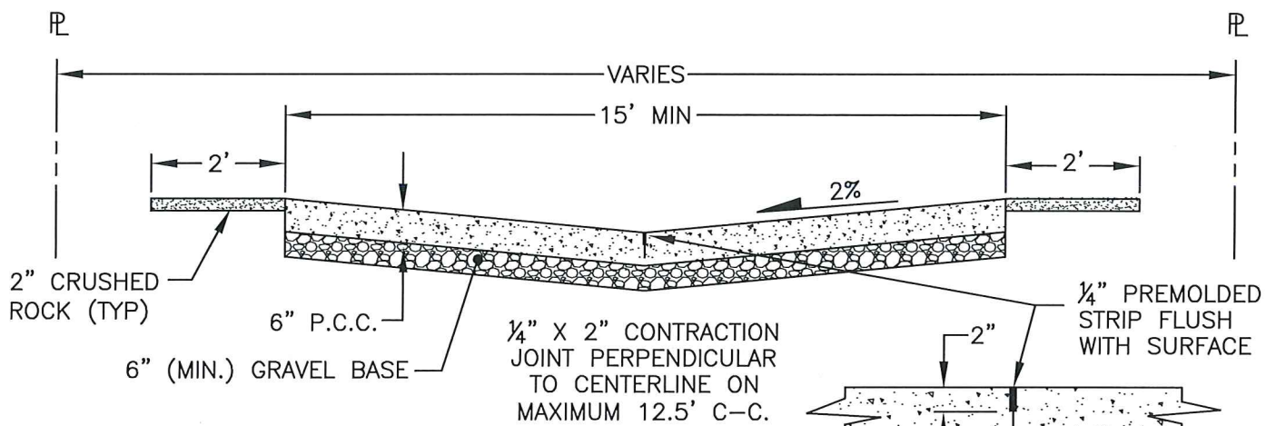
ALTERNATE B CEMENT CONCRETE ALLEY PAVEMENT
