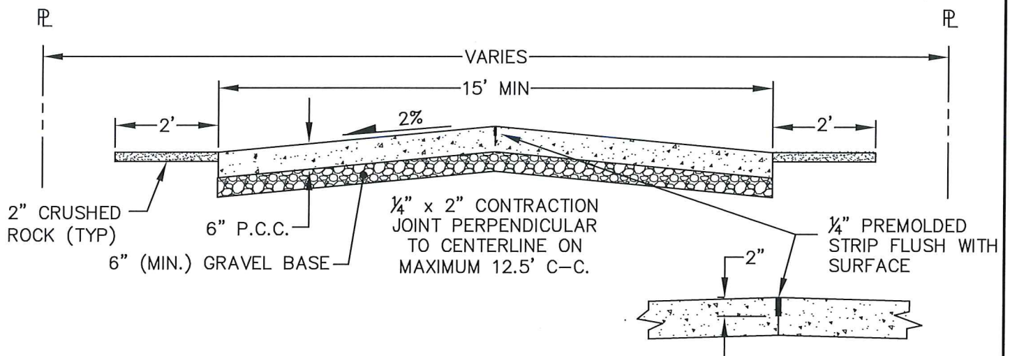
ALTERNATE B CEMENT CONCRETE ALLEY PAVEMENT
