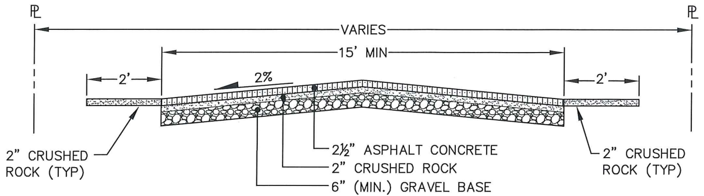
ALTERNATE A ASPHALT CONCRETE ALLEY PAVEMENT
