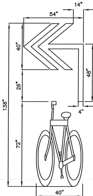
RIGHT OR LEFT TURN SHARED LANE MARKING (SLM) SYMBOL
