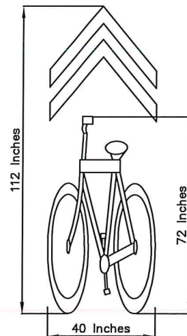
SHARED LANE MARKING (SLM) SYMBOL
