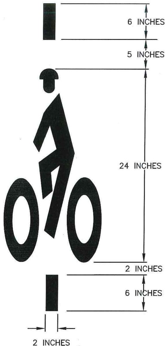
BICYCLE DETECTOR PAVEMENT MARKING
