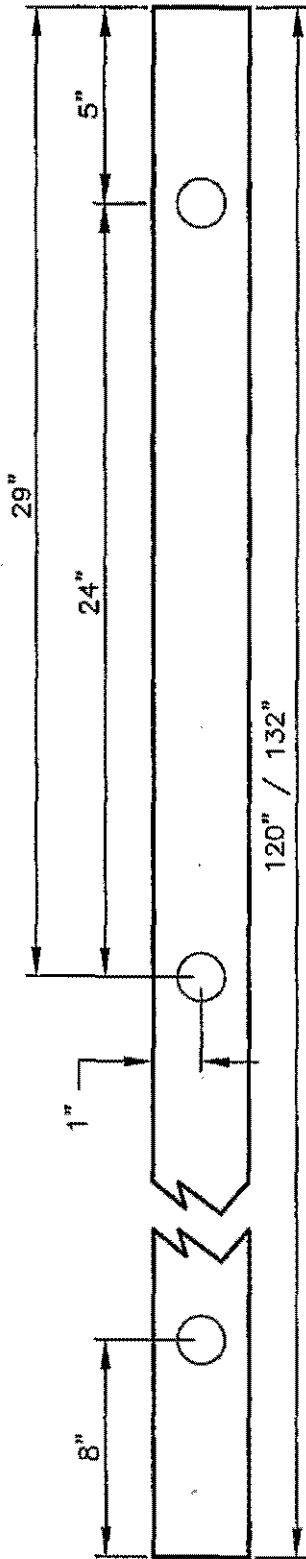
10 AND/OR 11 FT. SIGN POST
