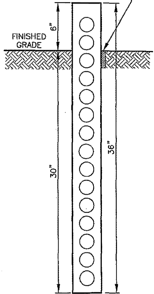
BASE PIECE
