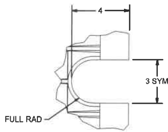
DETAIL D MOUSEHOLE DETAIL, THRU BOTH ENDS
