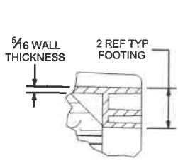
DETAIL C FOOTING DETAIL
