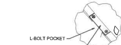
L-BOLT POCKET L-BOLT RETAINING PLATE (OPTIONAL, SOLD SEPARATELY) DETAIL E OPTIONAL L-BOLT RETAINING PLATE
