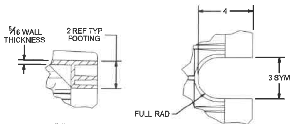
DETAIL C FOOTING DETAIL
