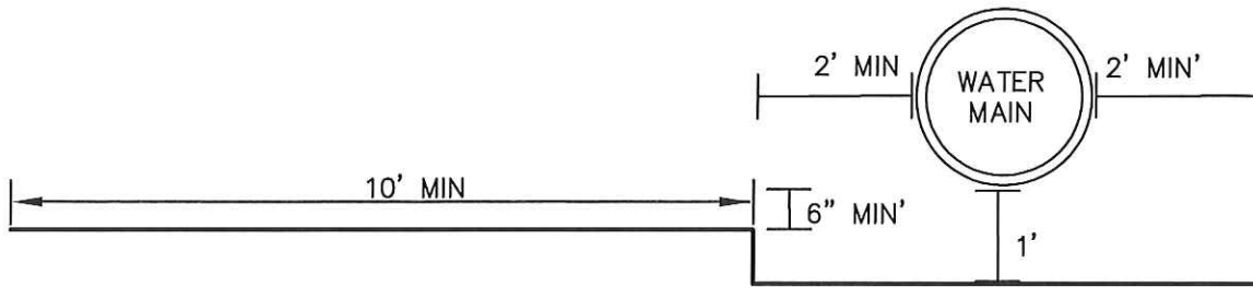
CROSS SECTION
