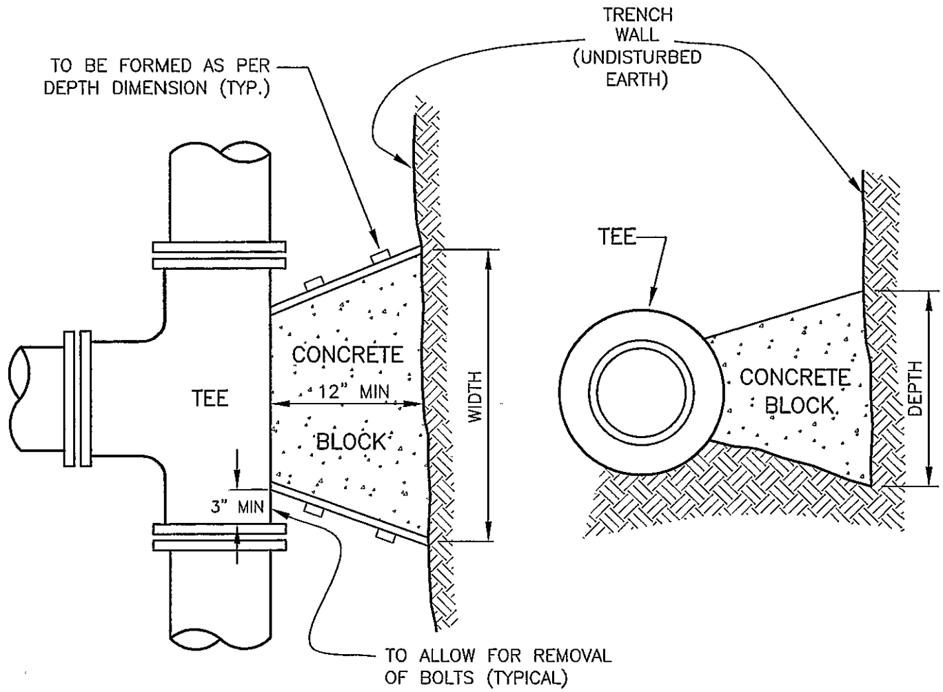
PLAN VIEW
