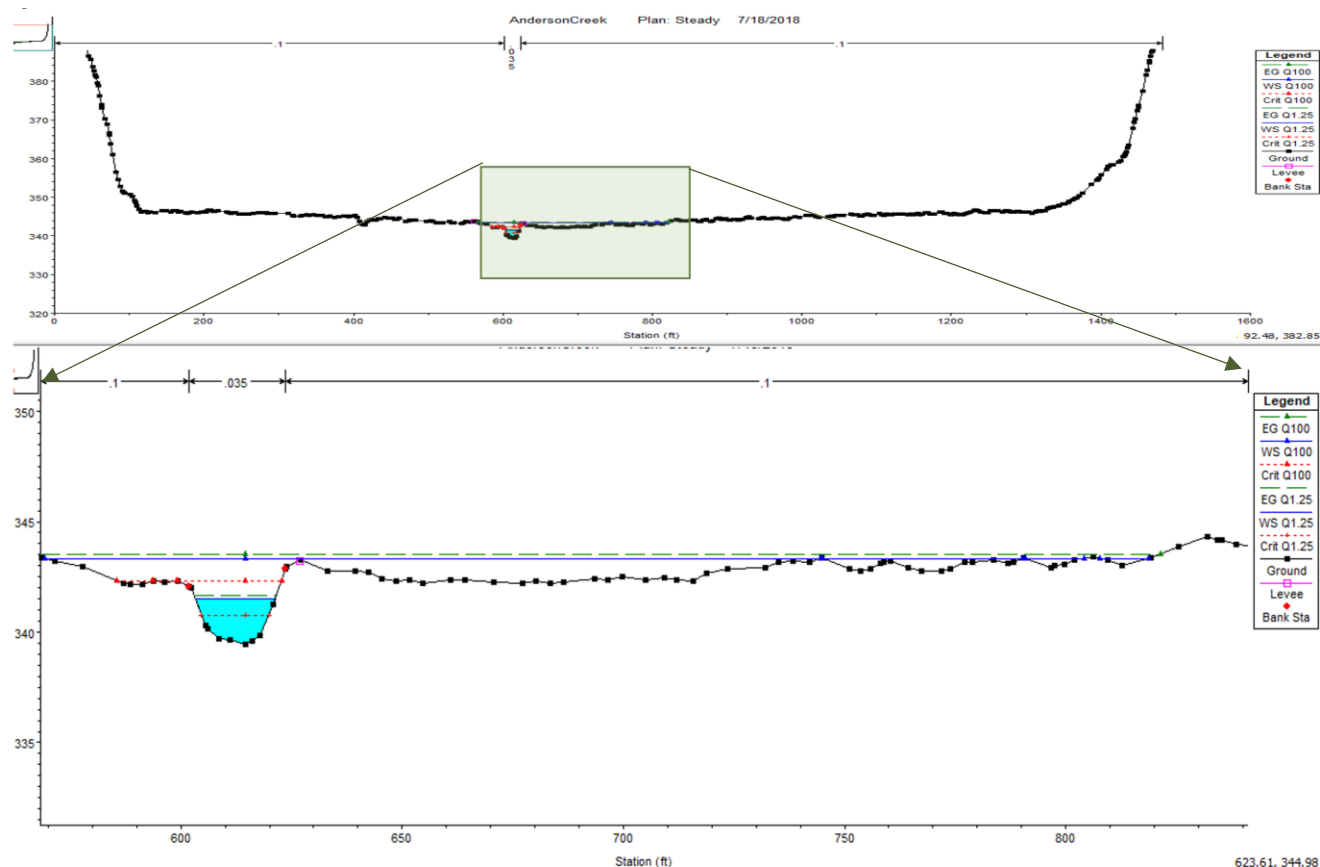
Figure 15. HEC-RAS results in Reach 5 showing broader inundation at the Q100 event.
