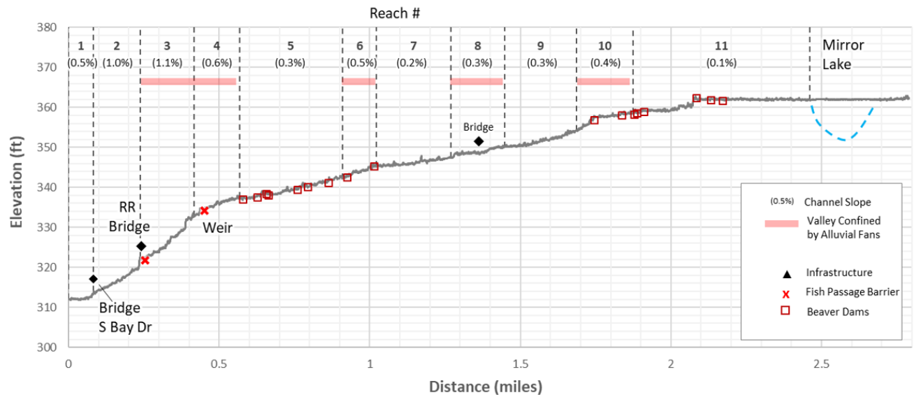
Figure 7. Anderson Creek Longitudinal profile from 2013 LiDAR showing the 11 geomorphic reaches.
