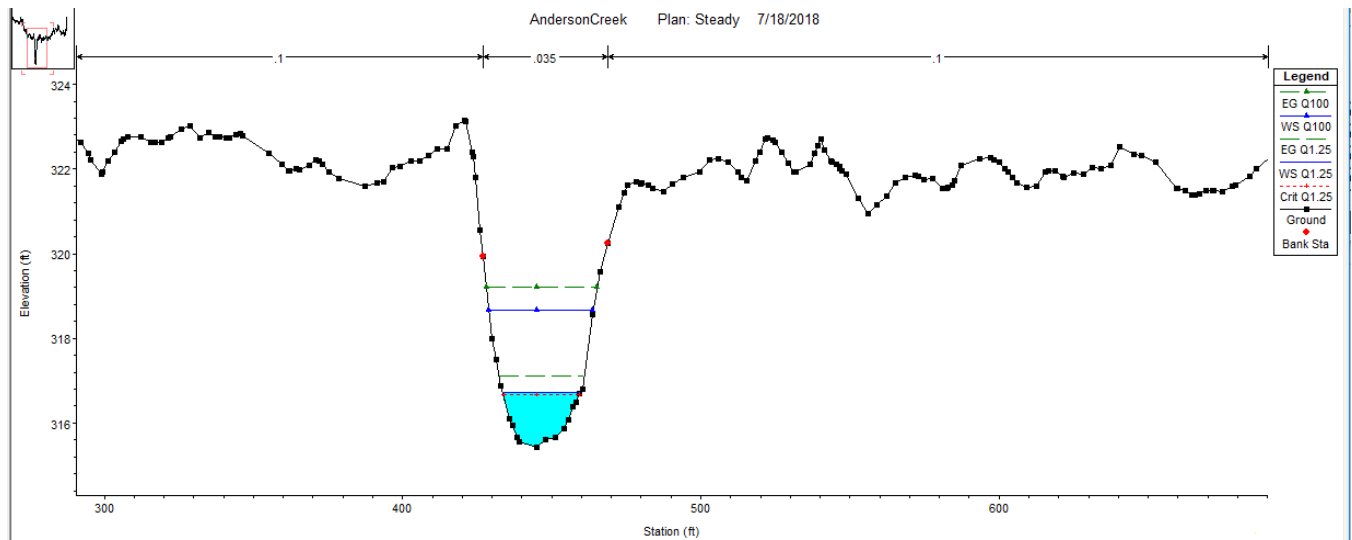
Figure 14. HEC-RAS results in Reach 2 showing the 1.25 year recurrence interval flow (Q1.25) in blue shading and the 100 year recurrence interval flow (Q100) stage in dark blue with triangles. Note that EG = Energy Grade, Crit = Depth at critical flow.
