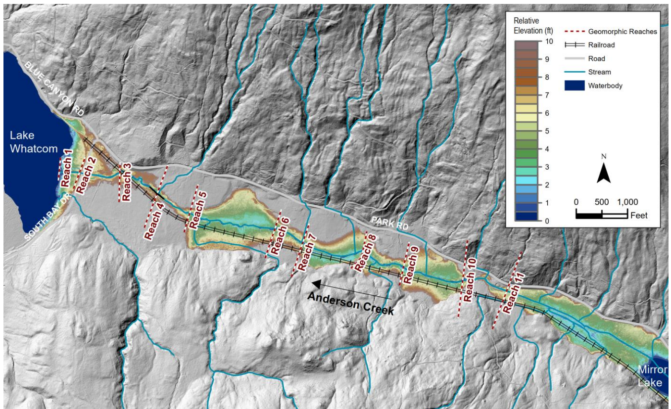
Figure 6. Relative Elevation Map of the Anderson Creek Valley. Relative elevations are based on the apparent water surface during the 2013 LiDAR data acquisition so the color ramp represents the floodplain elevation compared to the closest channel location.
