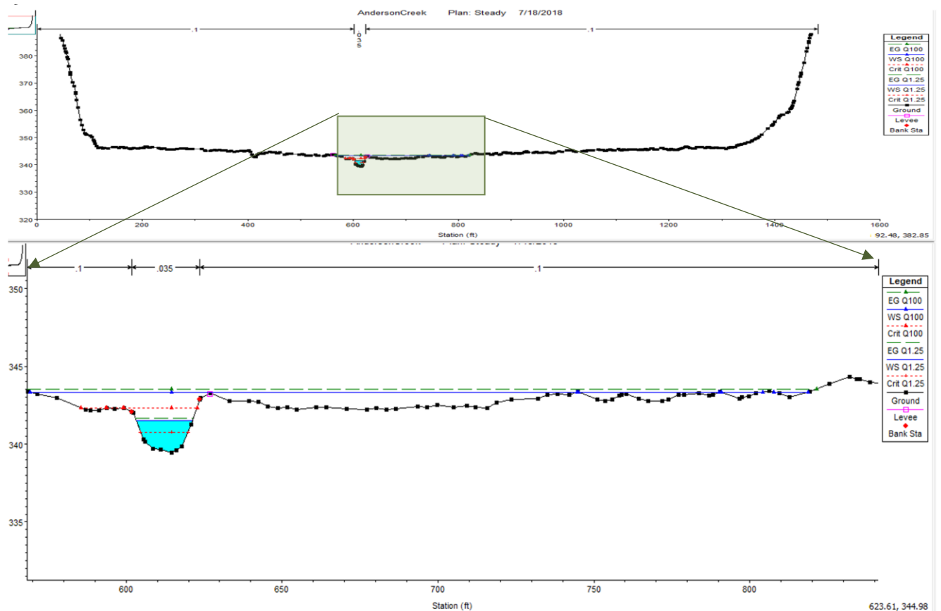
Figure 15. HEC-RAS results in Reach 5 showing broader inundation at the Q100 event.
