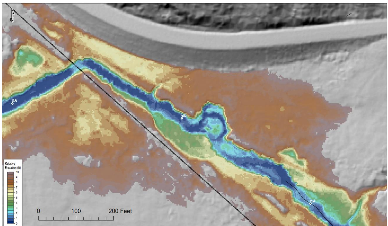
Figure 10. Relative elevation map showing new meander in Reach 3 formed due to erosion of the alluvial fan.
