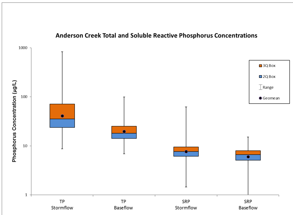
Figure 16. Phosphorus Concentrations in Anderson Creek ( note log scale )
