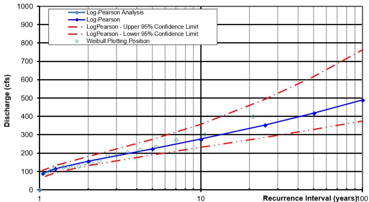
Figure 12 Log-Pearson analysis of flood recurrence intervals for Anderson Creek.
