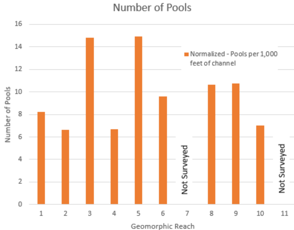
Figure 18. Normalized number of pools/1,000 feet of channel in Anderson Creek
