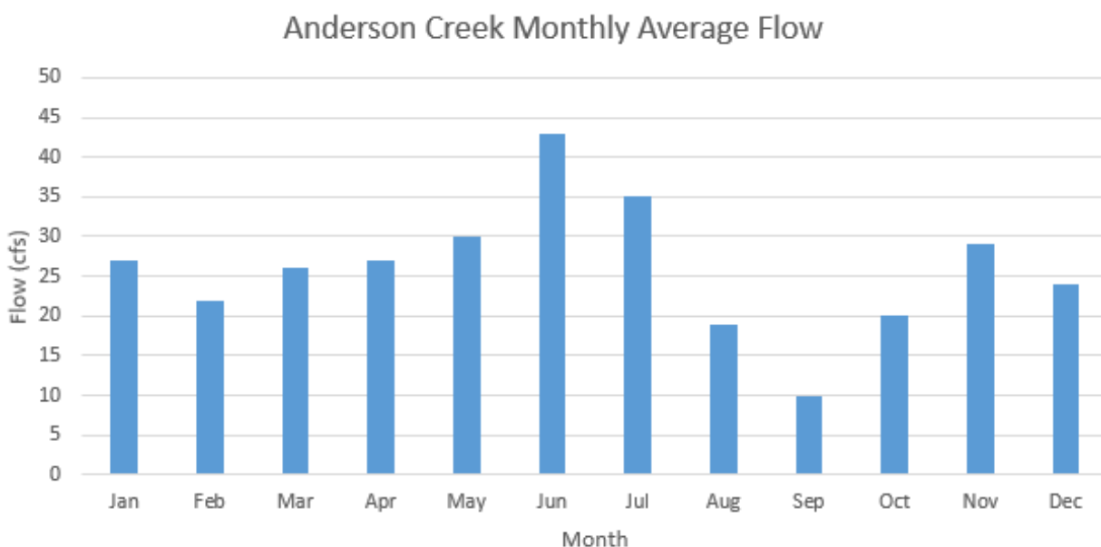
Figure 11 Anderson Creek hydrology shown as average monthly creek flow in cubic feet per second (cfs). Please note that these long-term statistics include diversion flows
