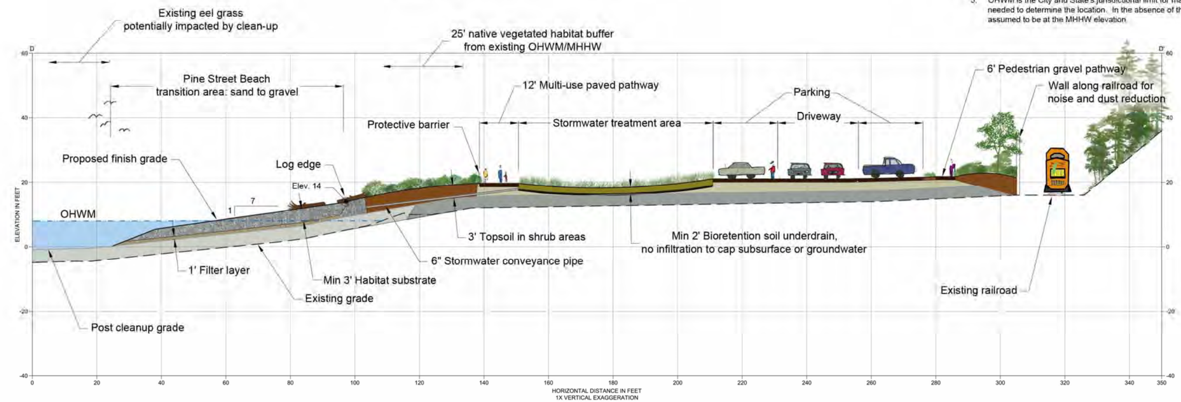
D Bioretention Swales Section D-D' (Pending Final Ecology Clean-up Remedy) Scale: 1" = 30.0'
