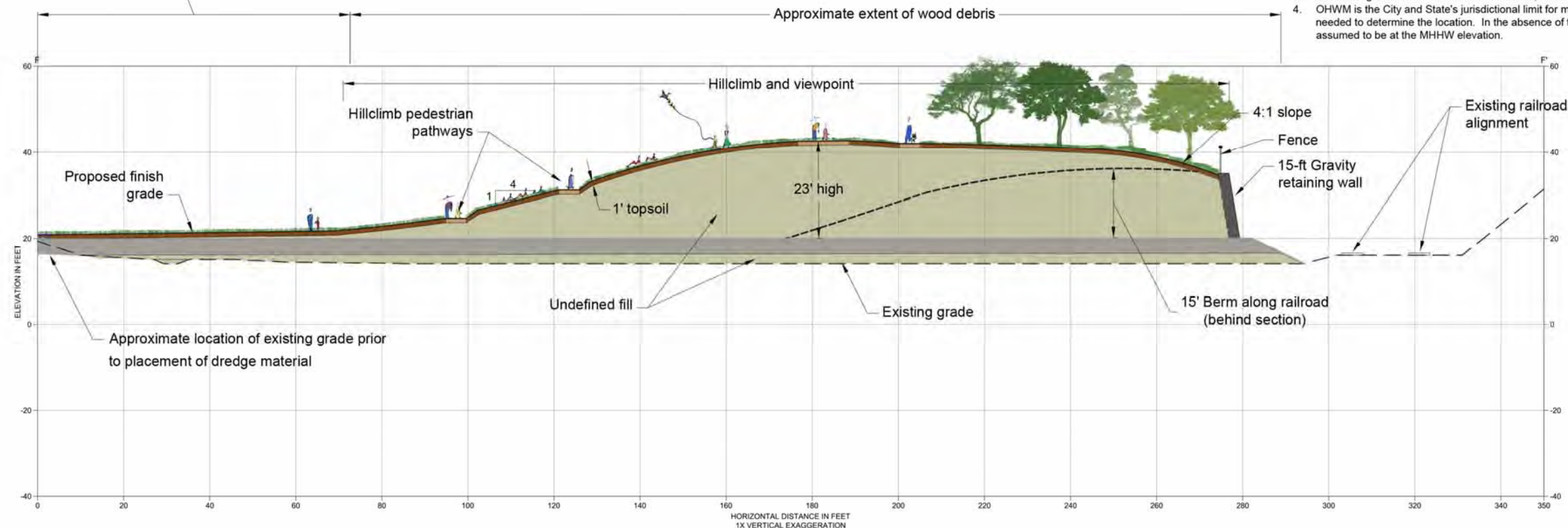
F Hill/Berm Section F-F' Scale: 1" = 30.0'
