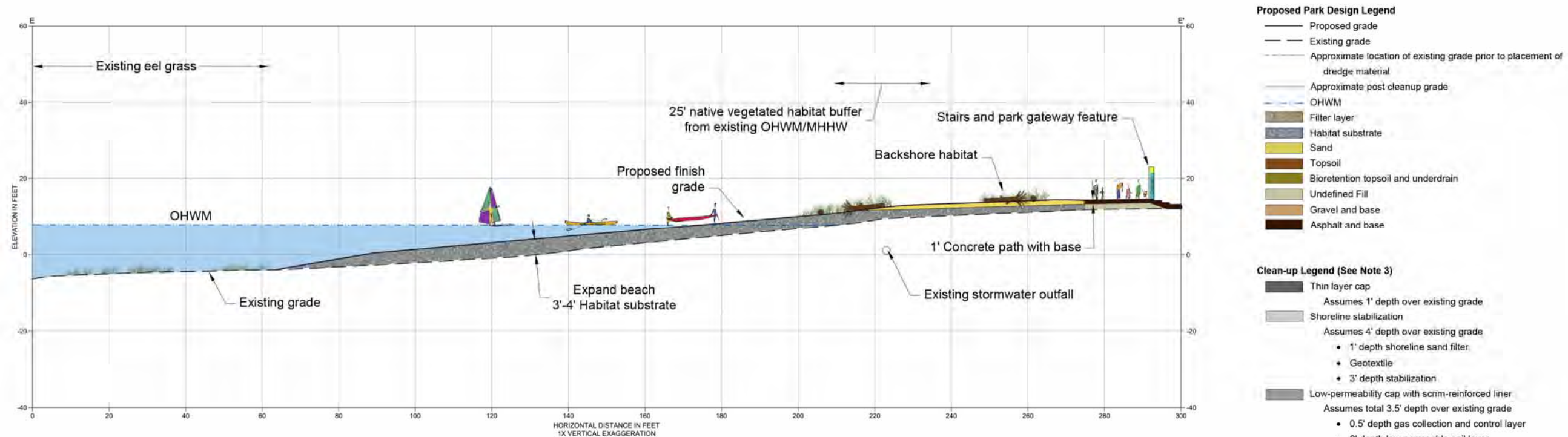
E Pine Street Beach Section E-E' Scale: 1" = 30.0'
