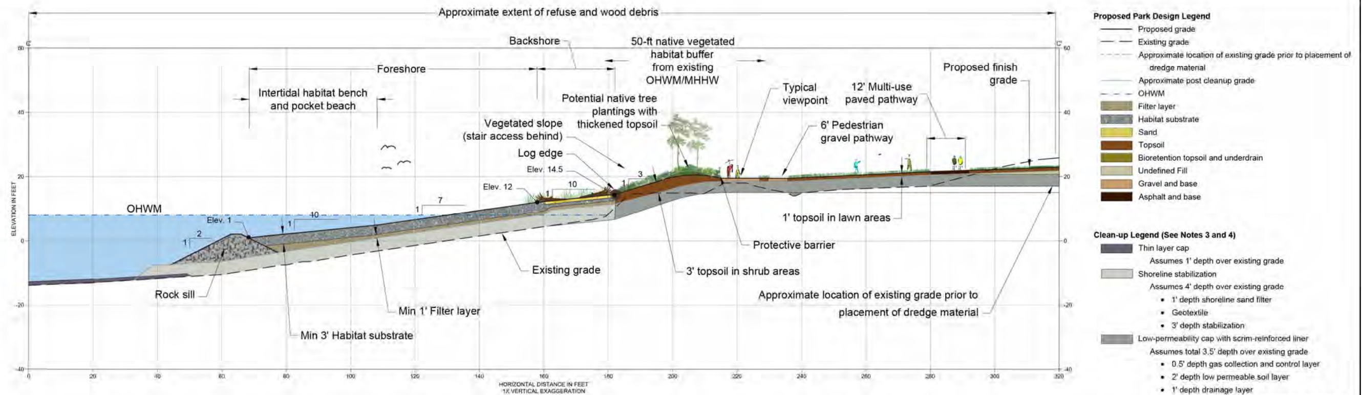
C Pocket Beach Section C-C' Scale: 1" = 30.0'
