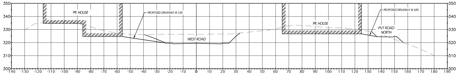
SECTION D-D SCALE H: 1"=20' V: 1=20'
