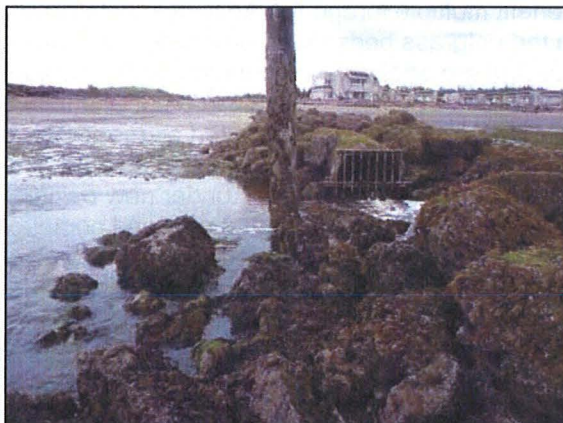
Figure 13. Culvert out-flow with considerable flow (CGS field photo).
