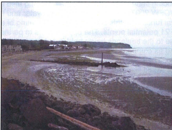
Figure 12. Looking east at armored culvert extending across shore (CGS field photo).
