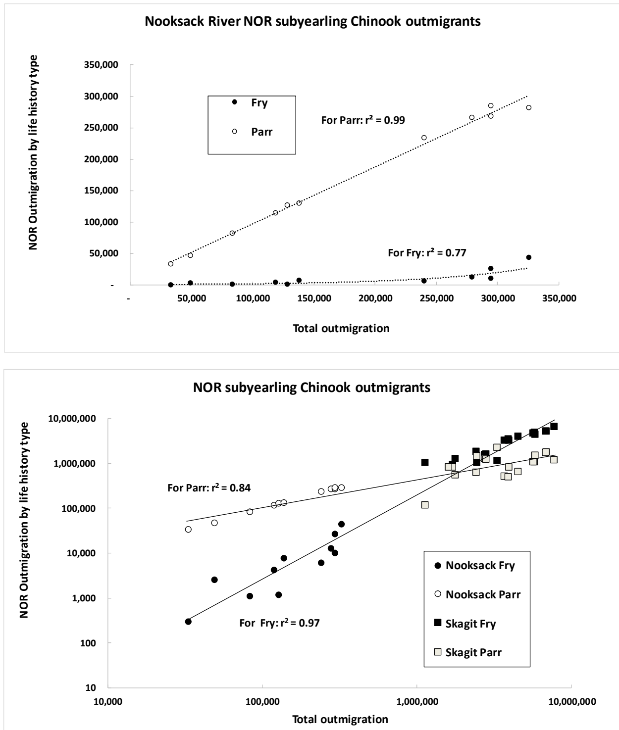
Figure 4.2.4. Expression of two NOR juvenile Chinook salmon life history strategies as a function of total subyearling outmigration size for the Nooksack River trapping years 2005 – 2015 (top panel) and Nooksack River and Skagit Rivers combined (bottom panel). Skagit data are for trapping years 1997 – 2015 (from Zimmerman et al. 2015 with additional years added courtesy J. Anderson and C. Kinsel of WDFW, pers. comm.).
