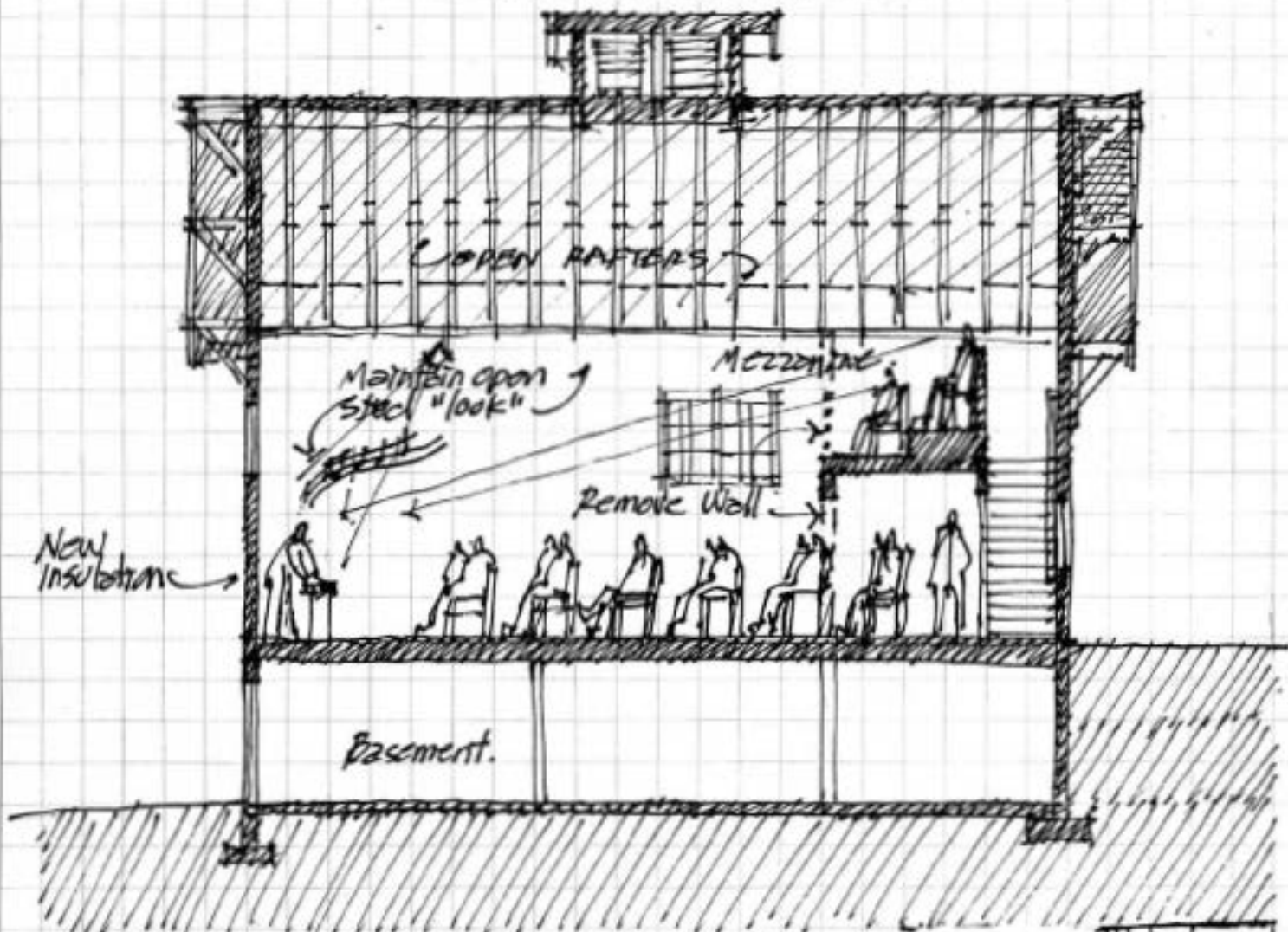
Building Section looking North at Barn
