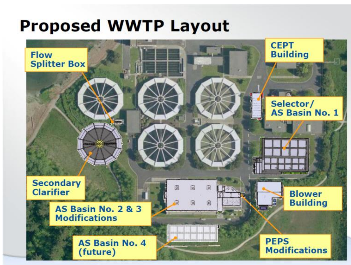
Figure 5: Post Point Waste Water Plant Expansion
