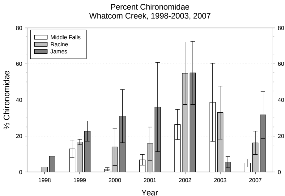
Figure 2-23. Mean relative abundances of the dipteran family Chironomidae in benthic macroinvertebrates samples collected at three sites on Whatcom Creek in Bellingham, Washington during September/ October, 1998-2003, and 2007. Error bars represent 95% confidence intervals.
